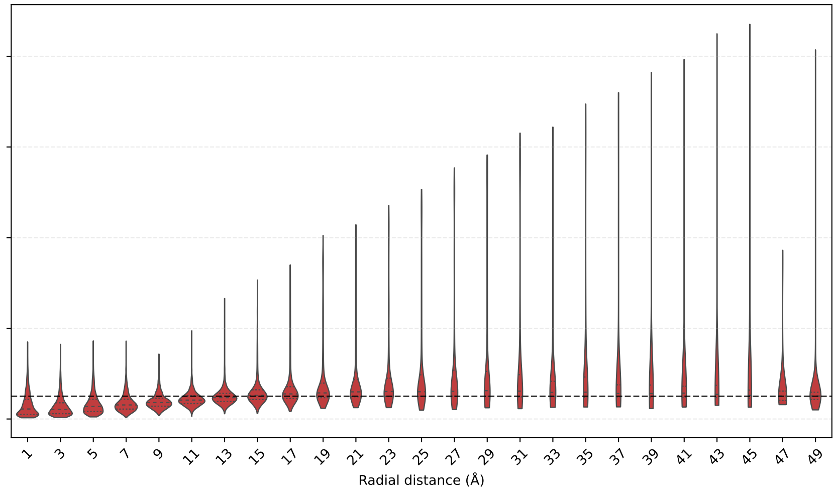
Physical RDF - radial distance in Å
