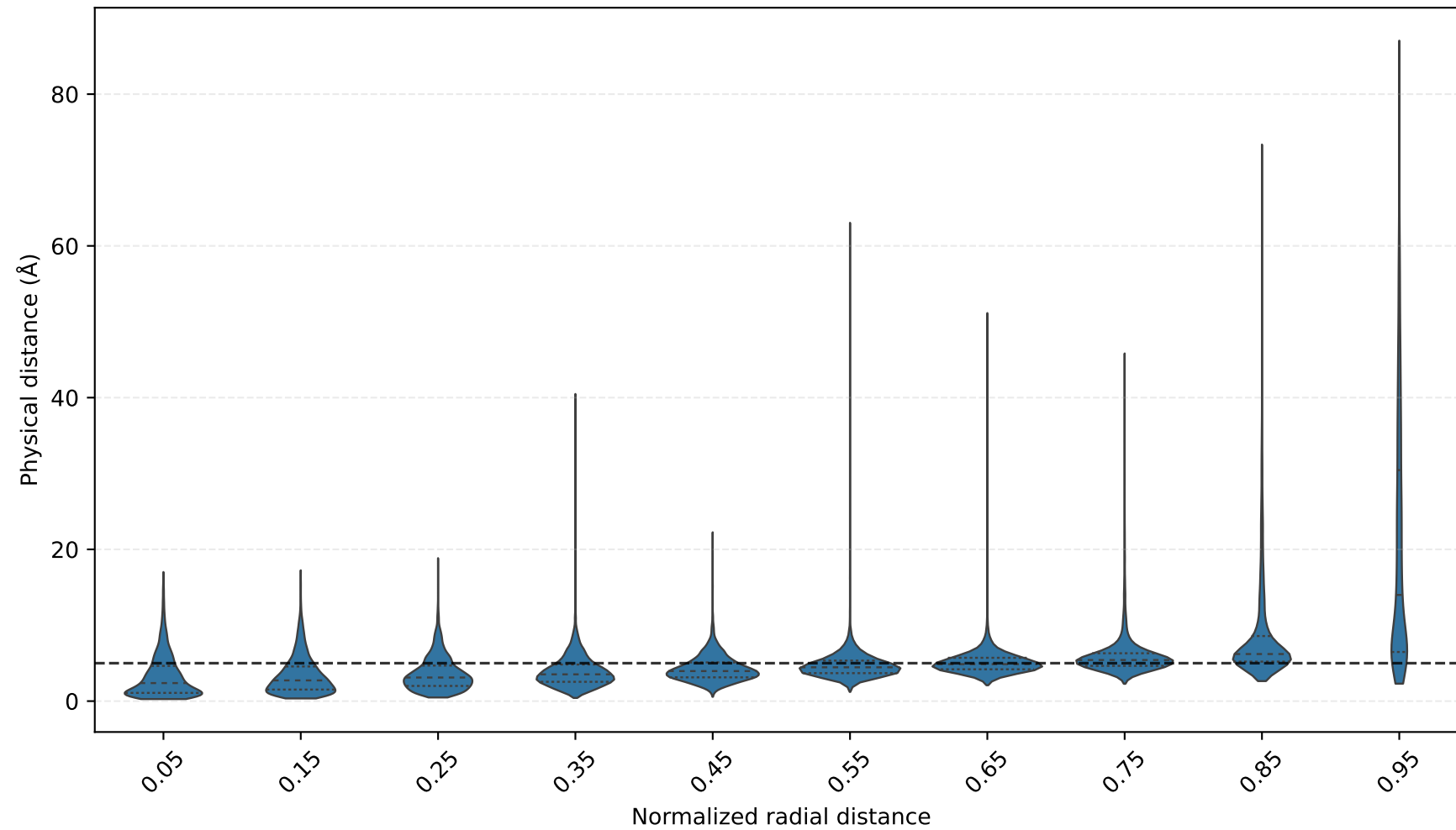
Physical RDF - normalized radial distance
