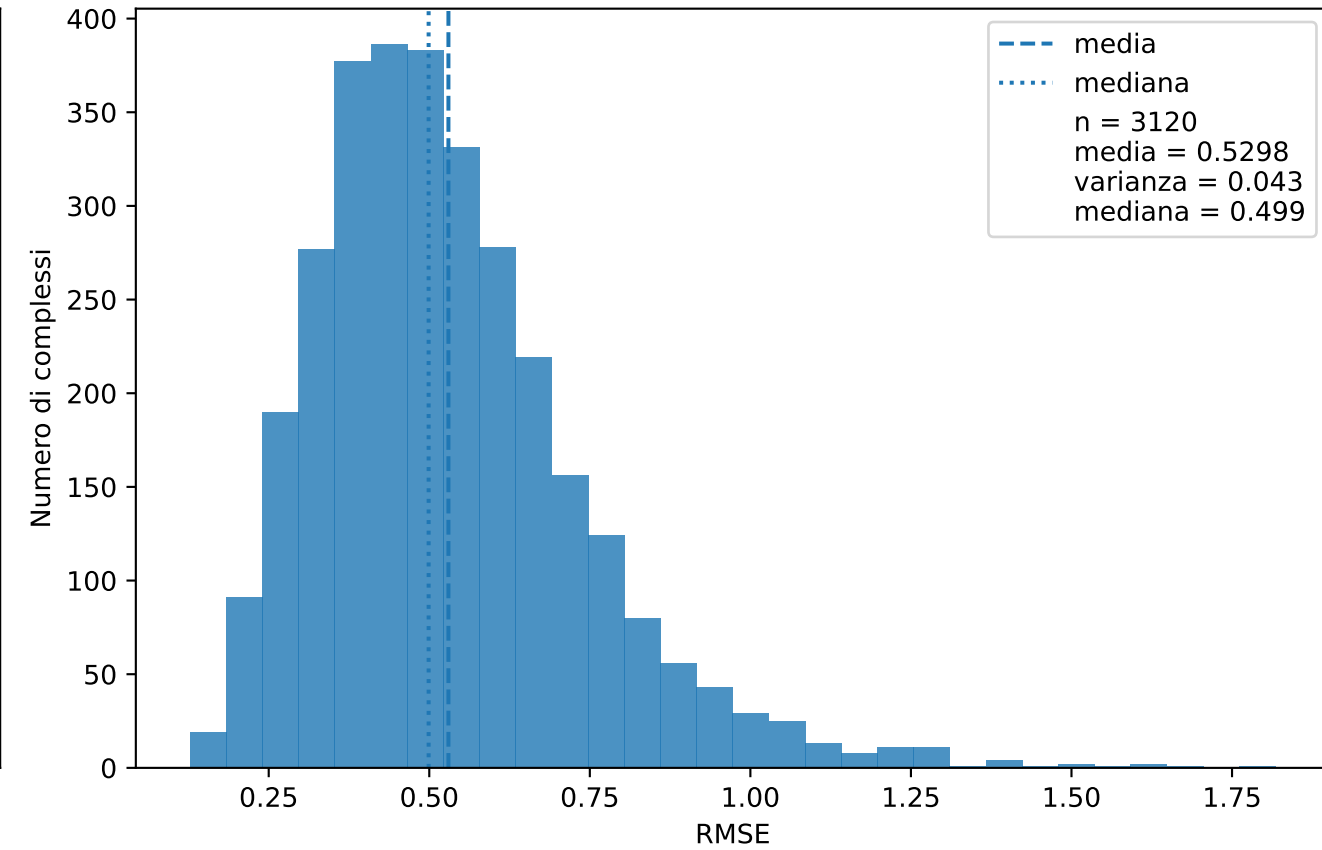
RMSE native-decoy (zernike)
