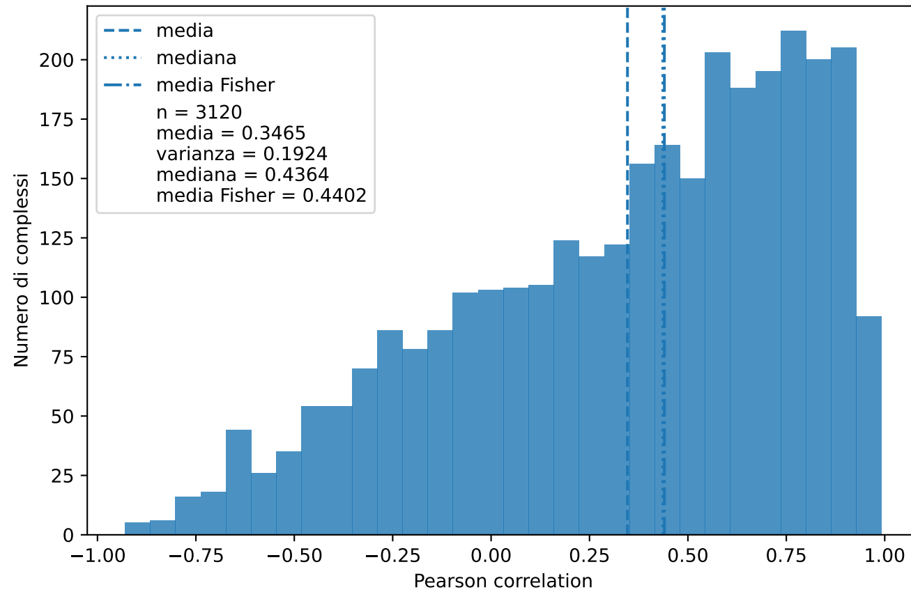
Pearson native-decoy (zernike)
