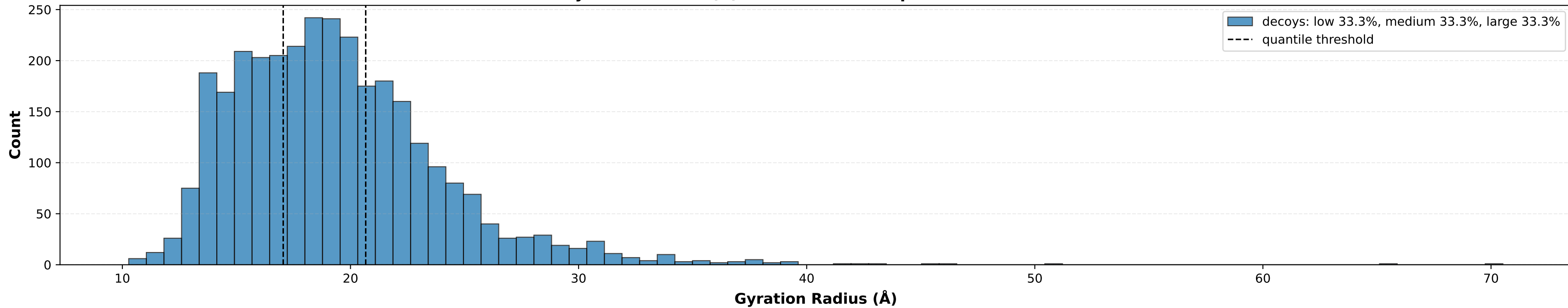
Gyration Radius (Å) - Physical Distance per Ring
