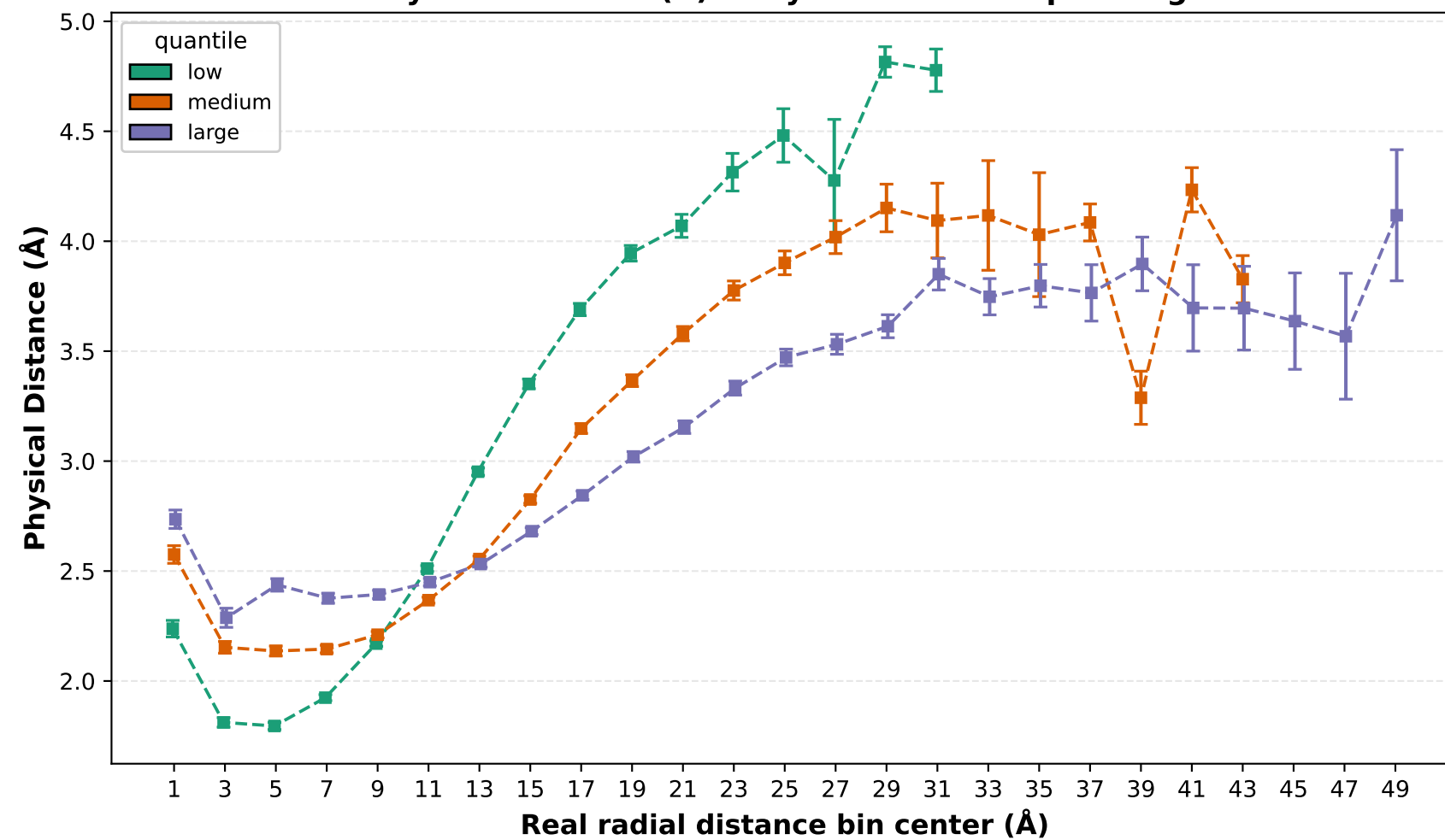
Gyration Radius (Å) - Physical Distance per Ring
