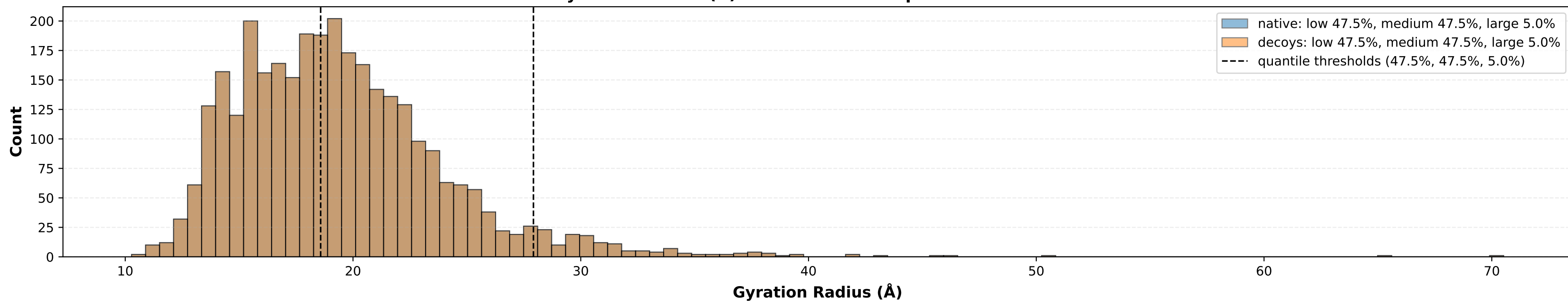
Gyration Radius (Å) - Low quantile - classical ring positions
