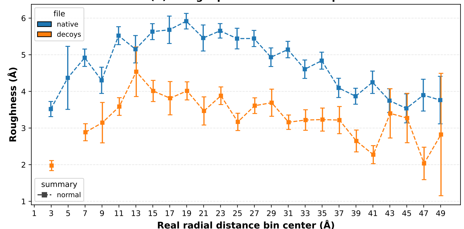
Radius (Å) - Large quantile - real radial positions
