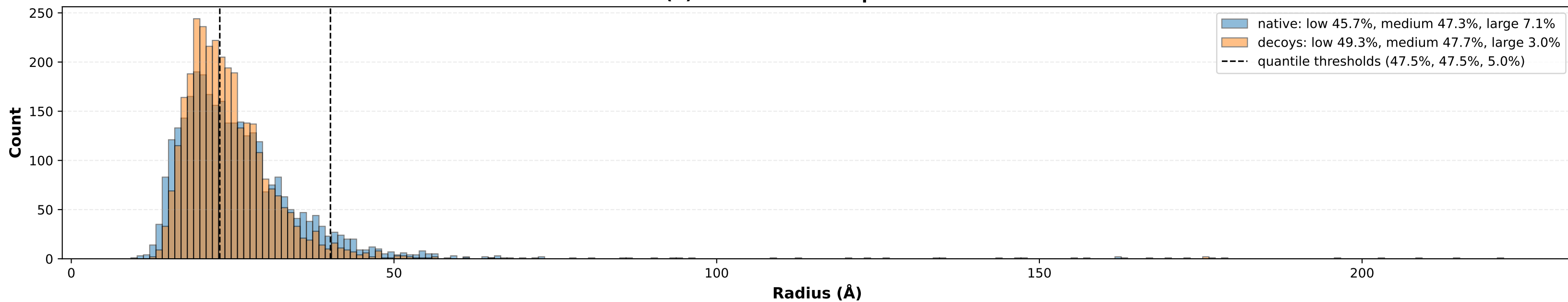
Radius (Å) - Low quantile - classical ring positions
