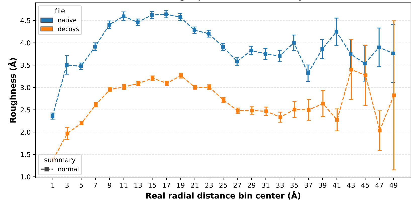
Radius (Å) - Large quantile - real radial positions
