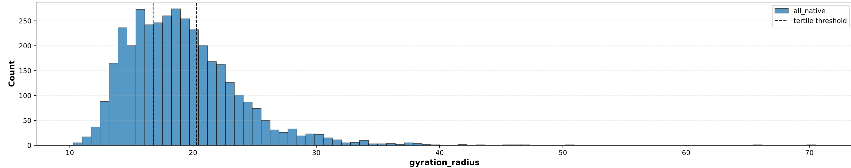
gyration_radius - Physical Distance per Ring
