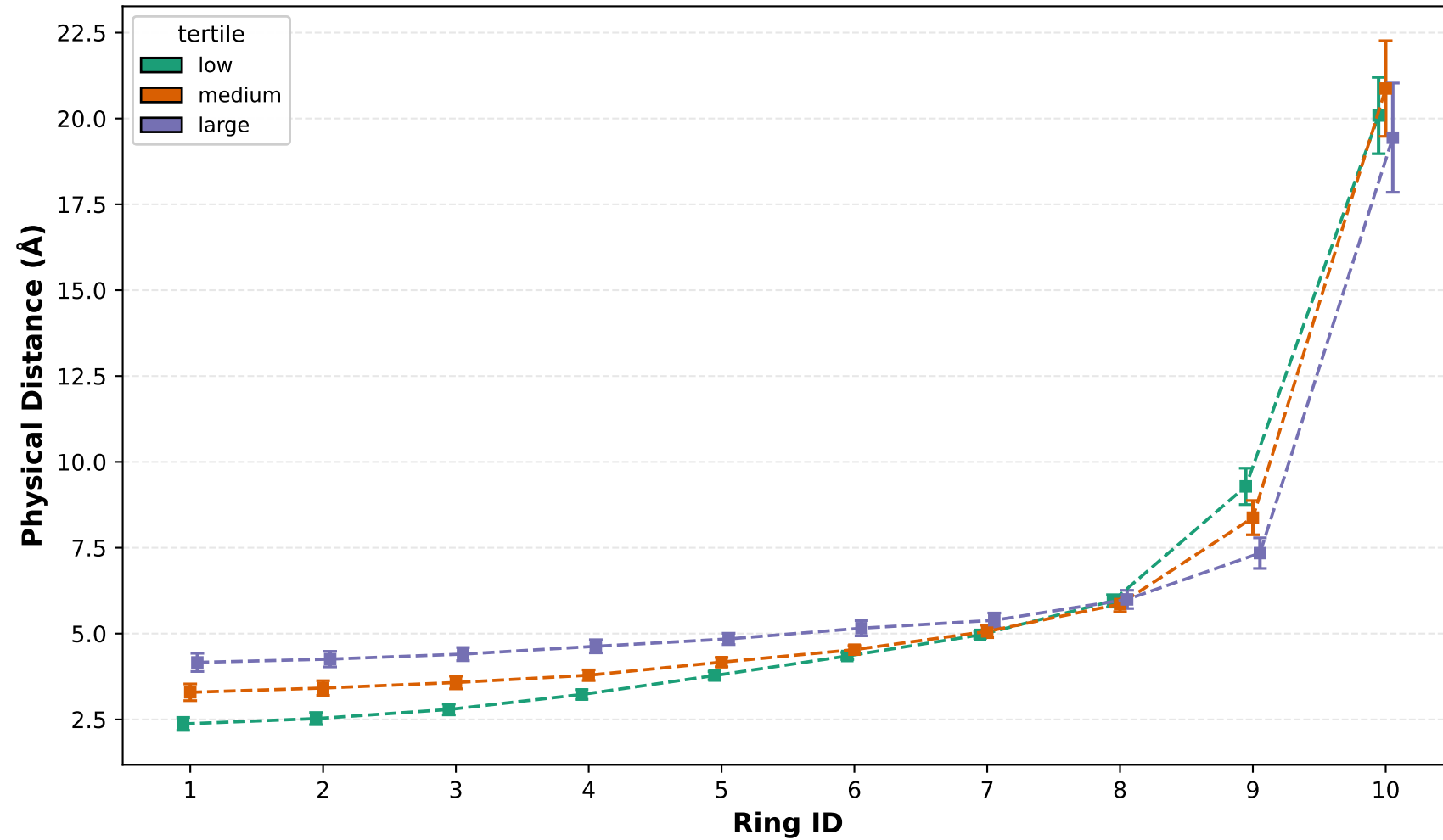
gyration_radius - Physical Distance per Ring
