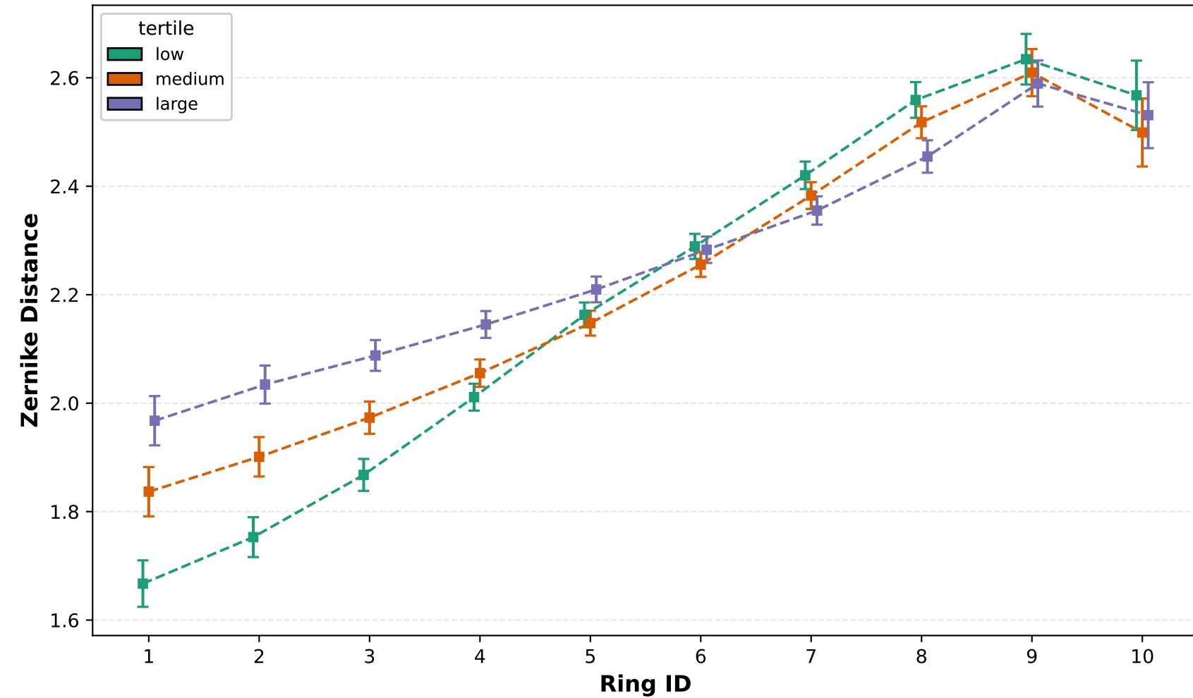
gyration_radius - Zernike Distance per Ring
