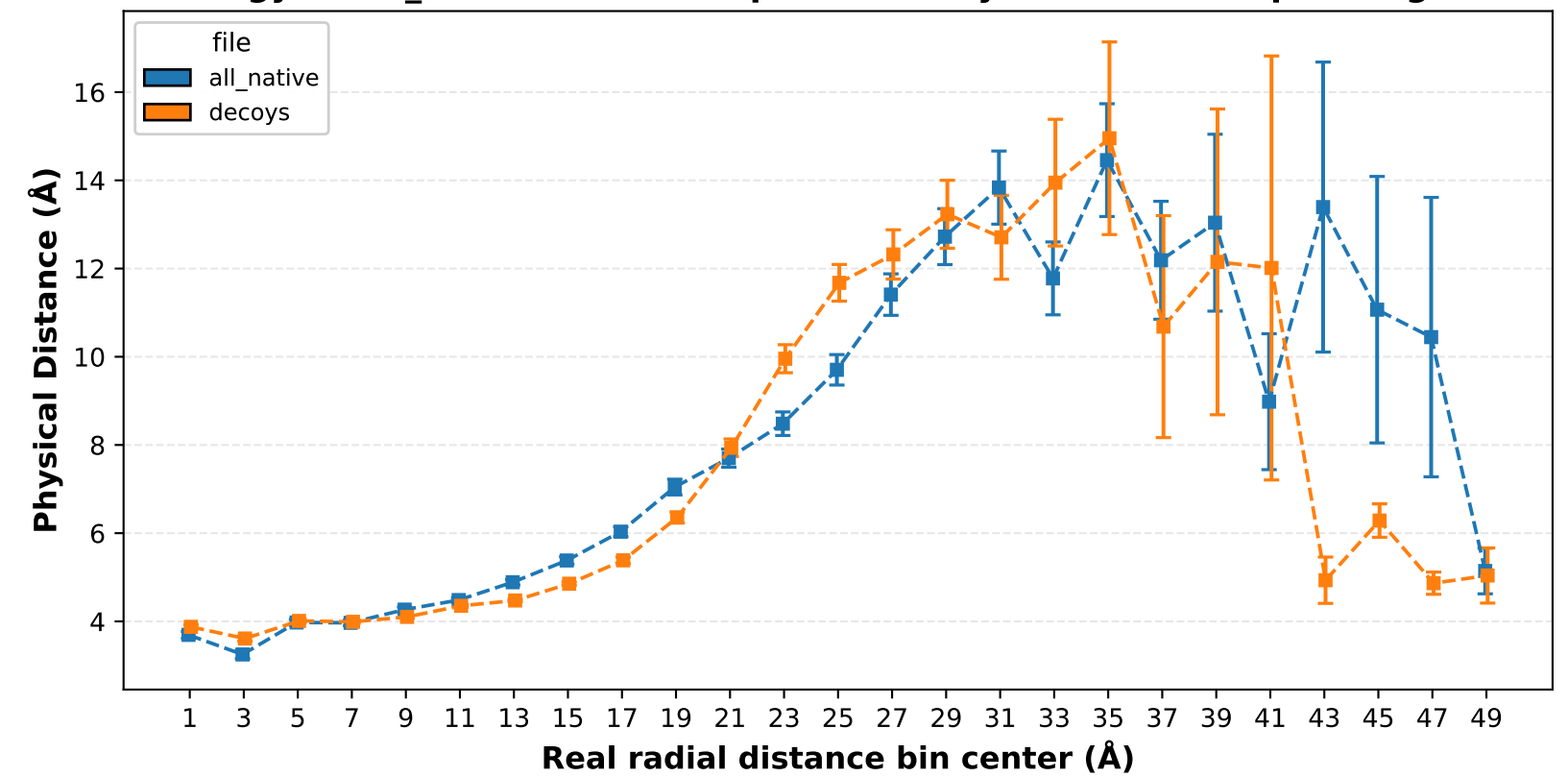
gyration_radius - Large quantile - Physical Distance per Ring
