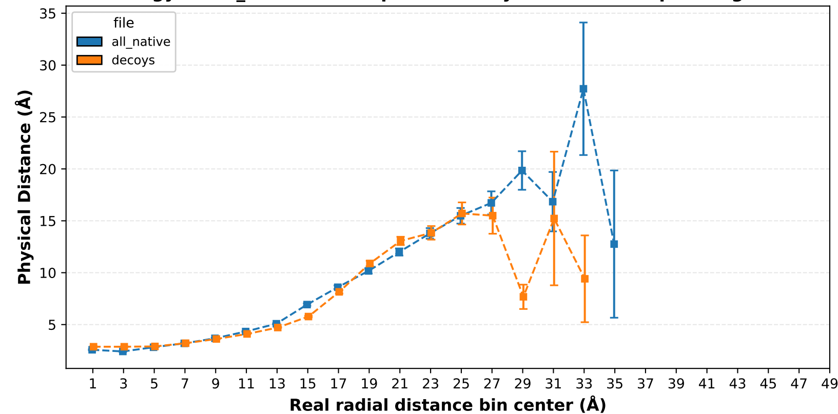
gyration_radius - Medium quantile - Physical Distance per Ring
