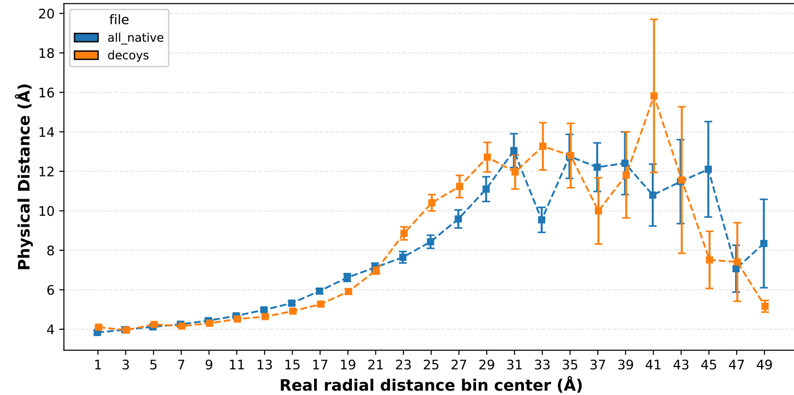
gyration_radius - Large tertile - Physical Distance per Ring
