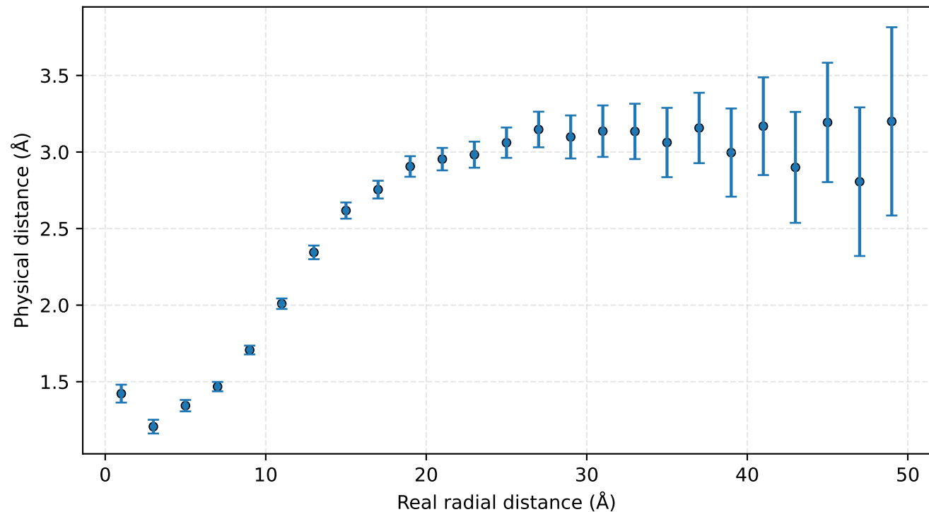
Real radial distance (2Å bins)
