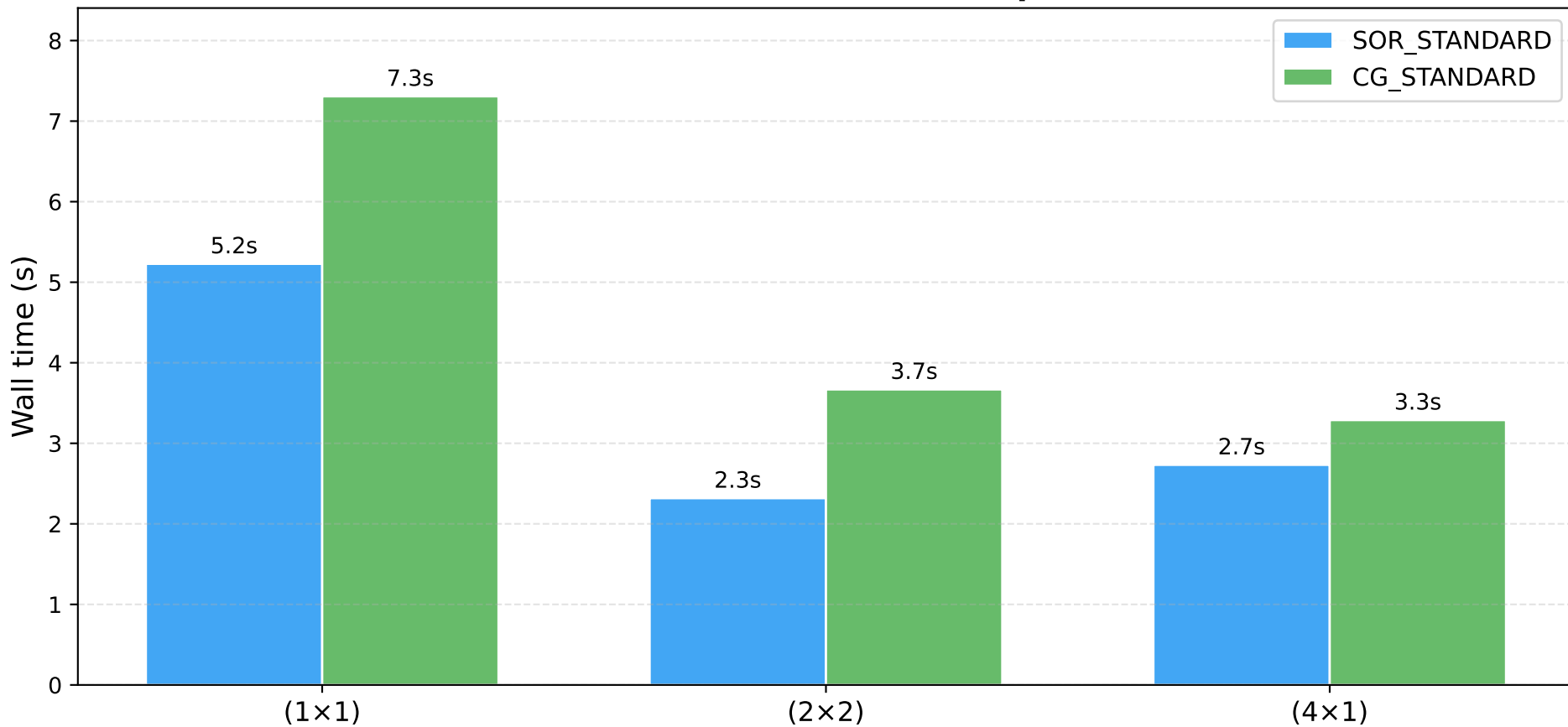
Wall time: SOR vs CG — Fluid Trap (100×50)
