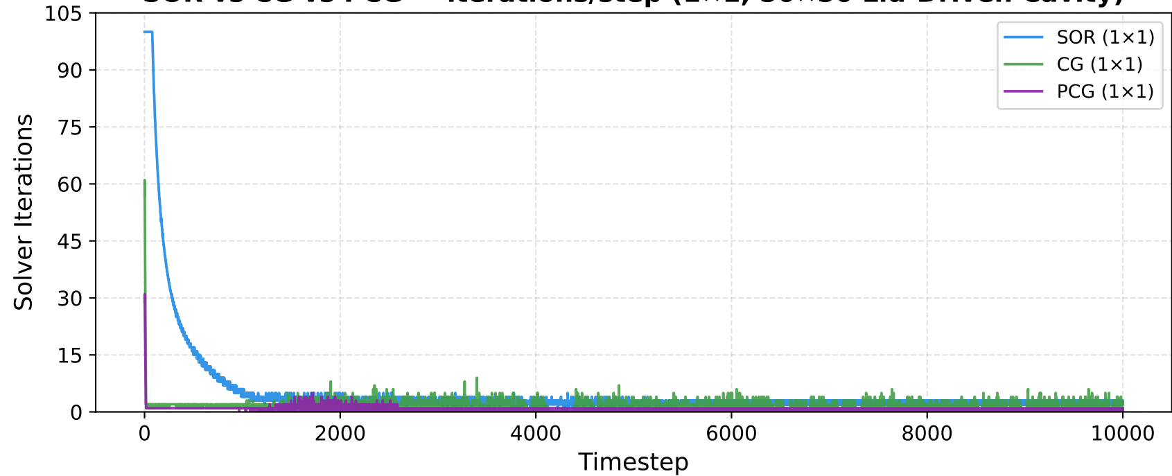
SOR vs CG vs PCG — iterations/step ( 1\times 1 , 50\times 50 Lid-Driven Cavity)
