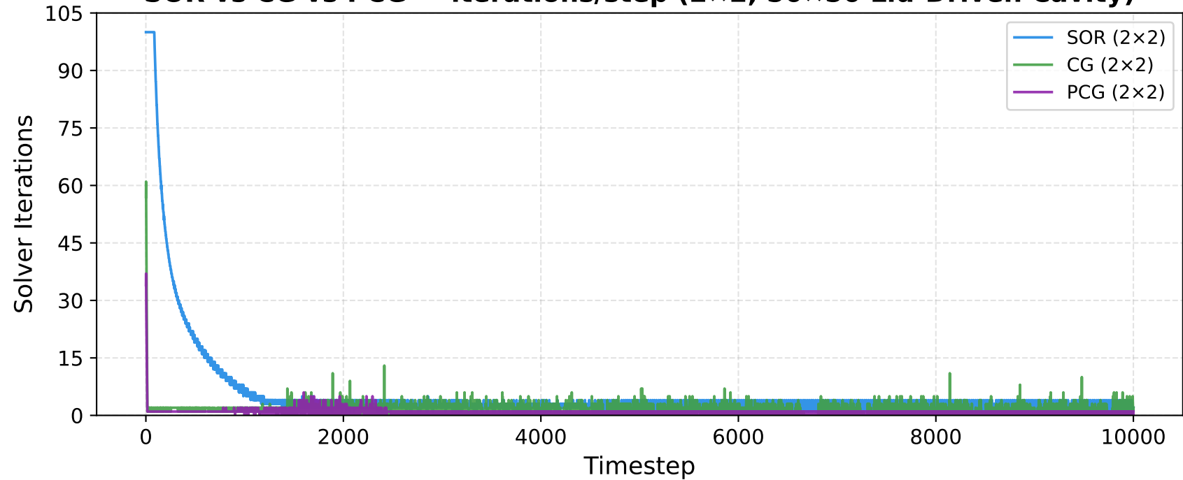
SOR vs CG vs PCG — iterations/step ( 2\times 2 , 50\times 50 Lid-Driven Cavity)
