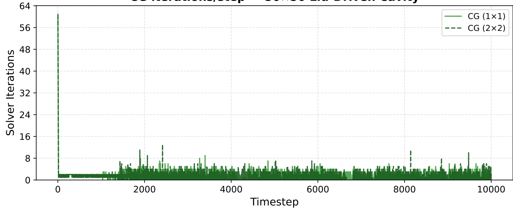
CG iterations/step — 50×50 Lid-Driven Cavity
