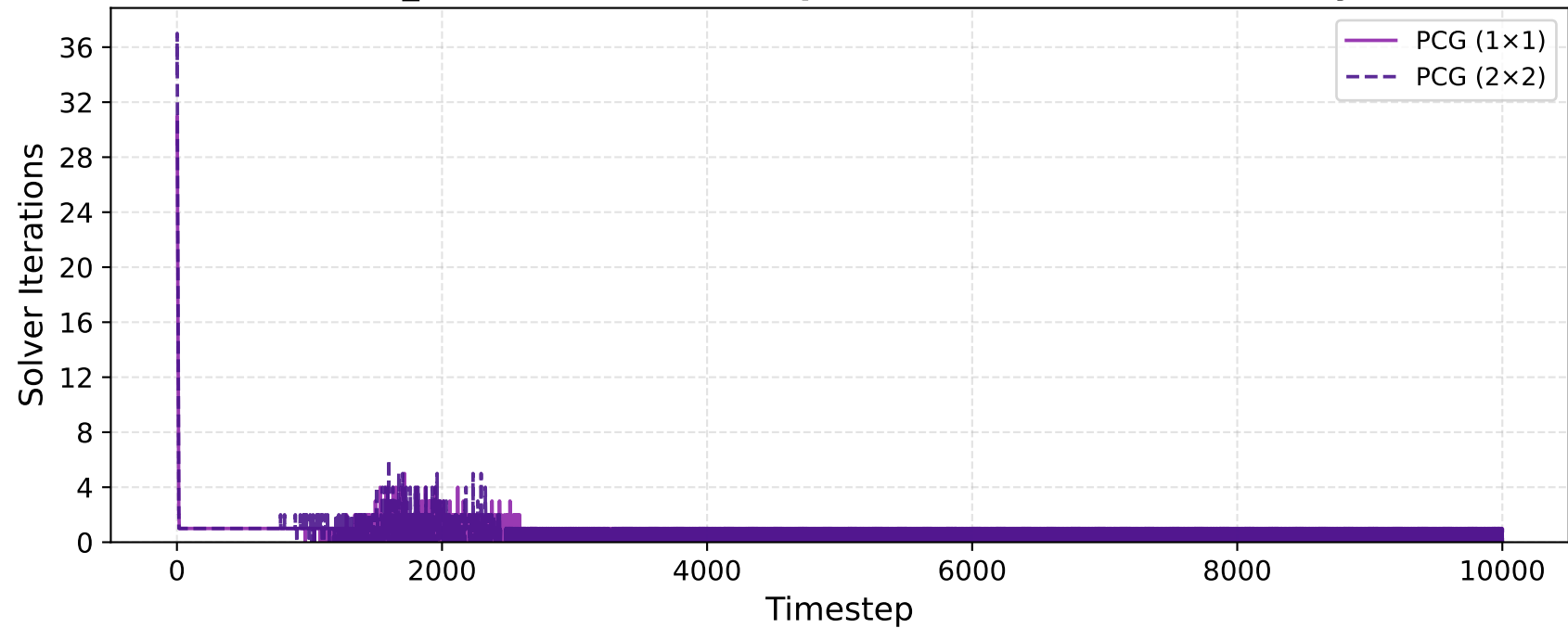
PCG_SSOR iterations/step — 50×50 Lid-Driven Cavity
