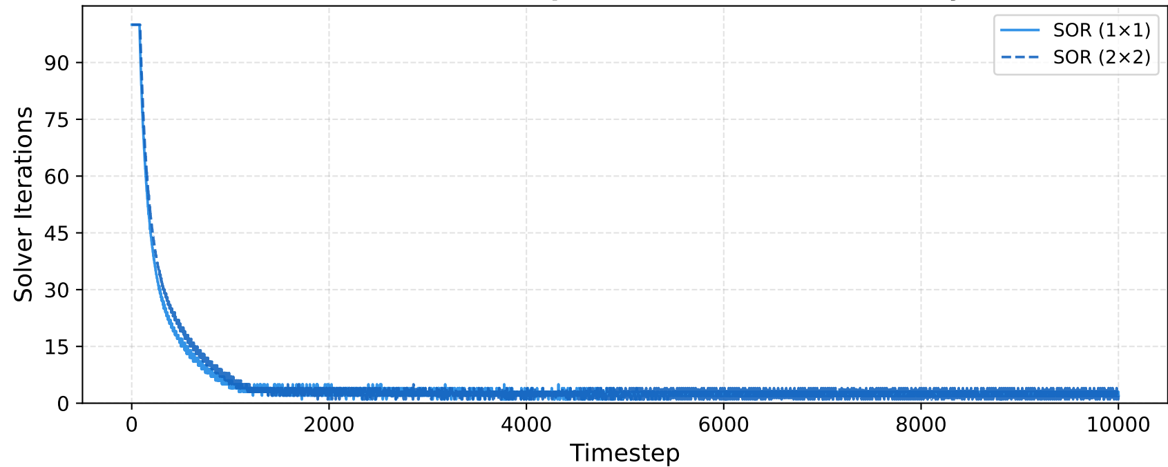
SOR iterations/step — 50×50 Lid-Driven Cavity
