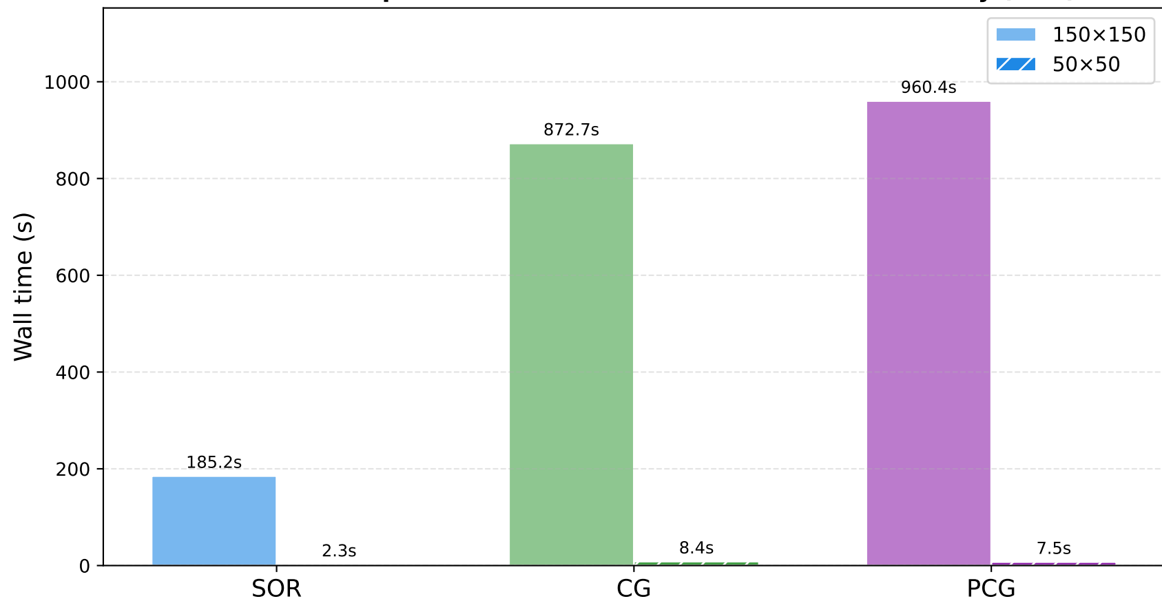
Wall time comparison: 50×50 vs 150×150 Lid-Driven Cavity (1×1)
