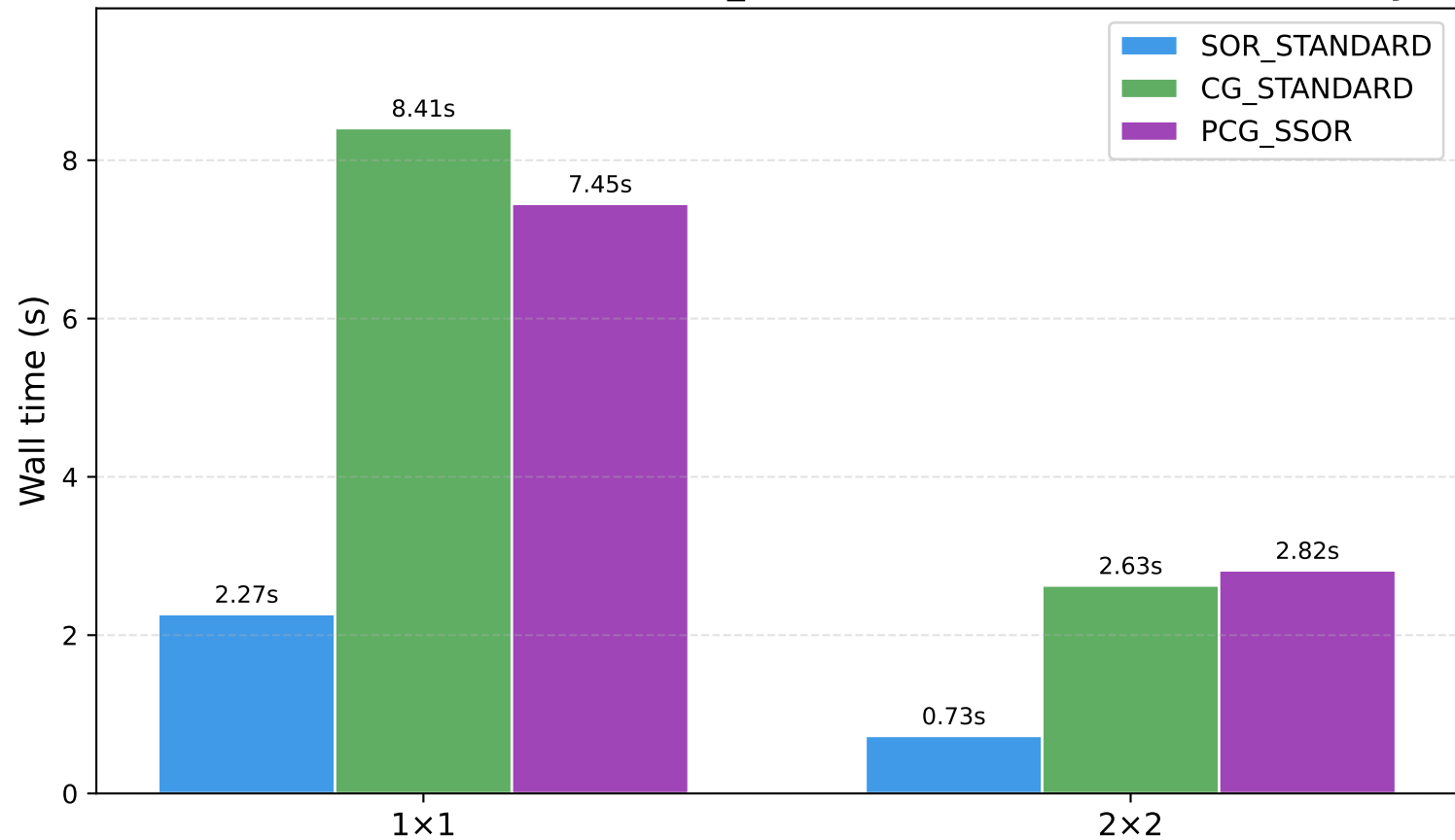
Wall time: SOR vs CG vs PCG_SSOR — 50×50 Lid-Driven Cavity
