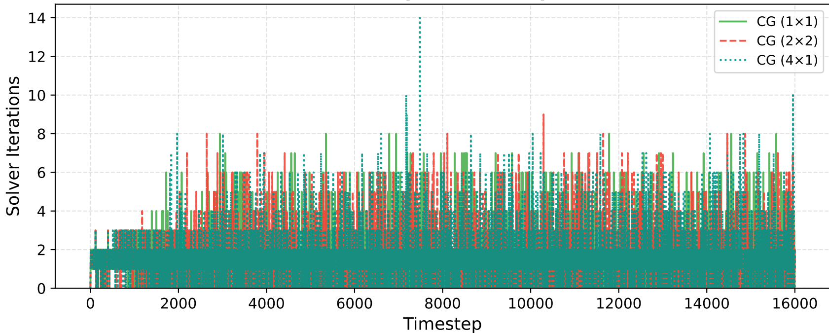
CG iterations/step — Fluid Trap (100×50)
