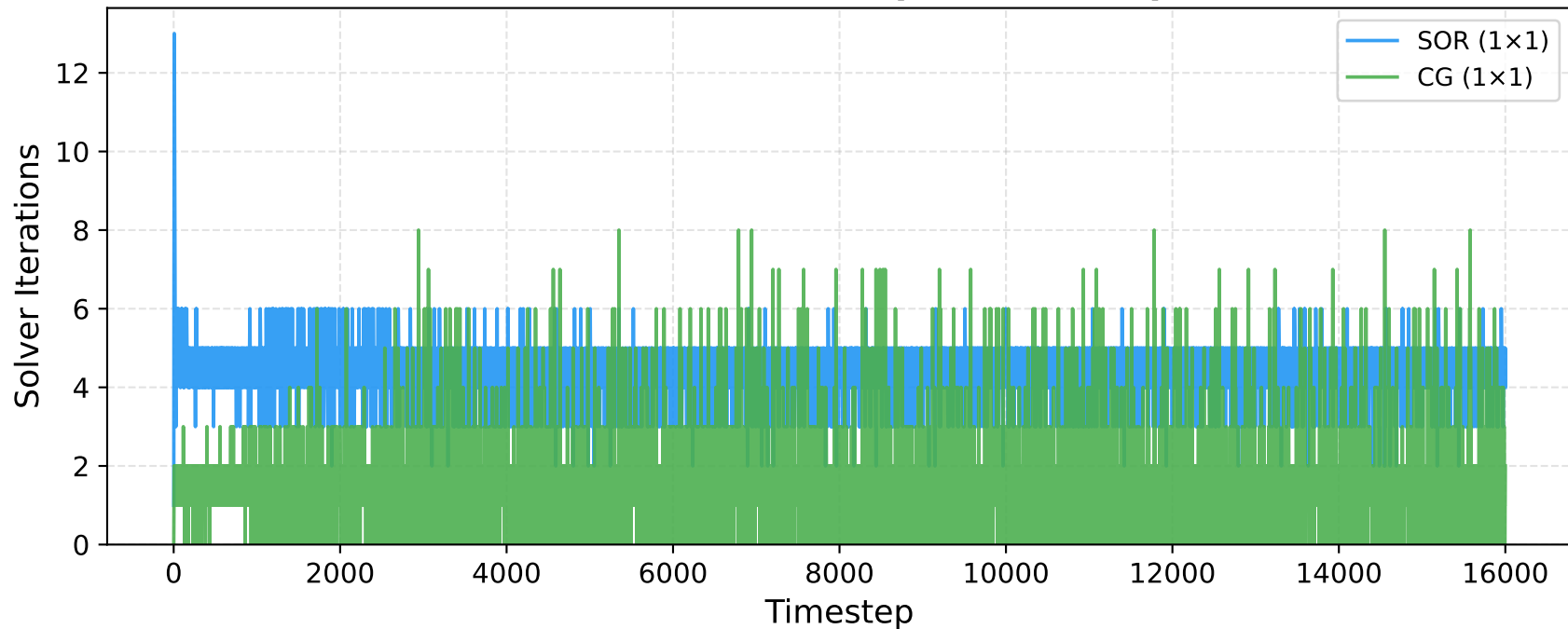
SOR vs CG iterations/step — Fluid Trap 1×1
