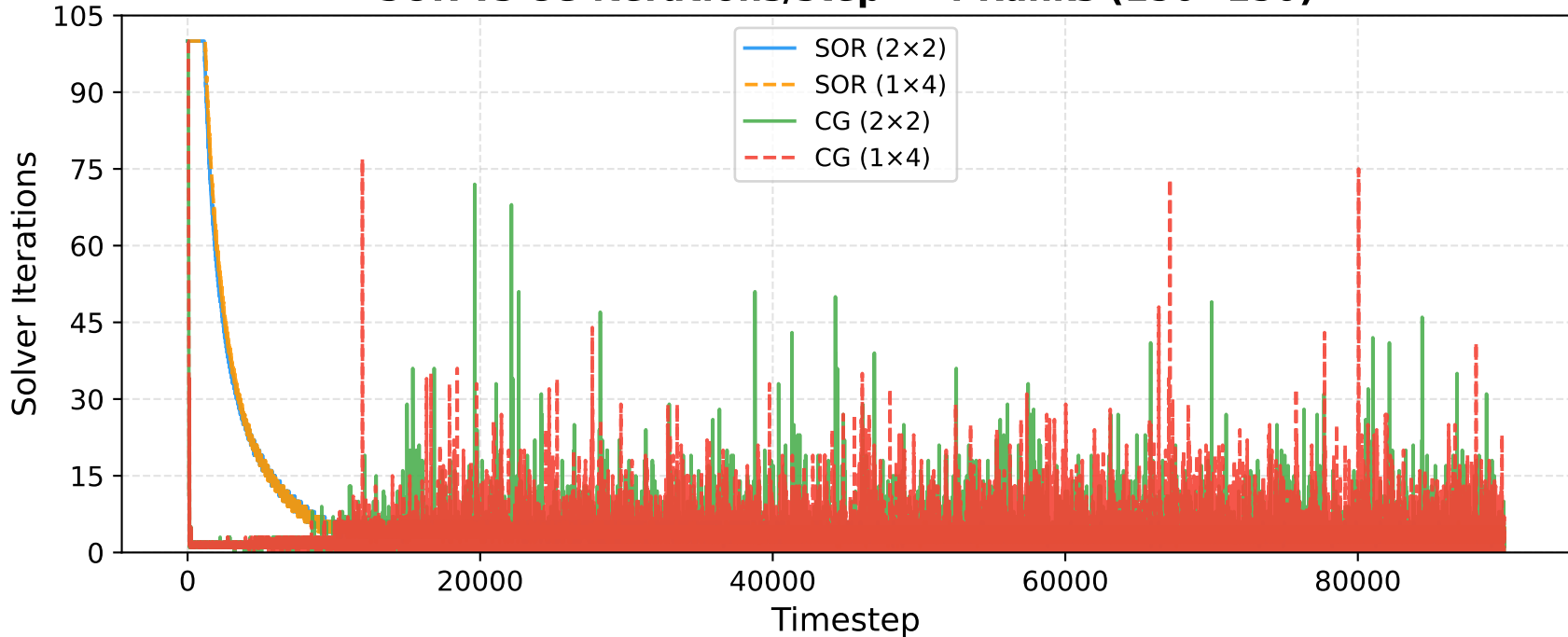
SOR vs CG iterations/step — 4 Ranks (150×150)
