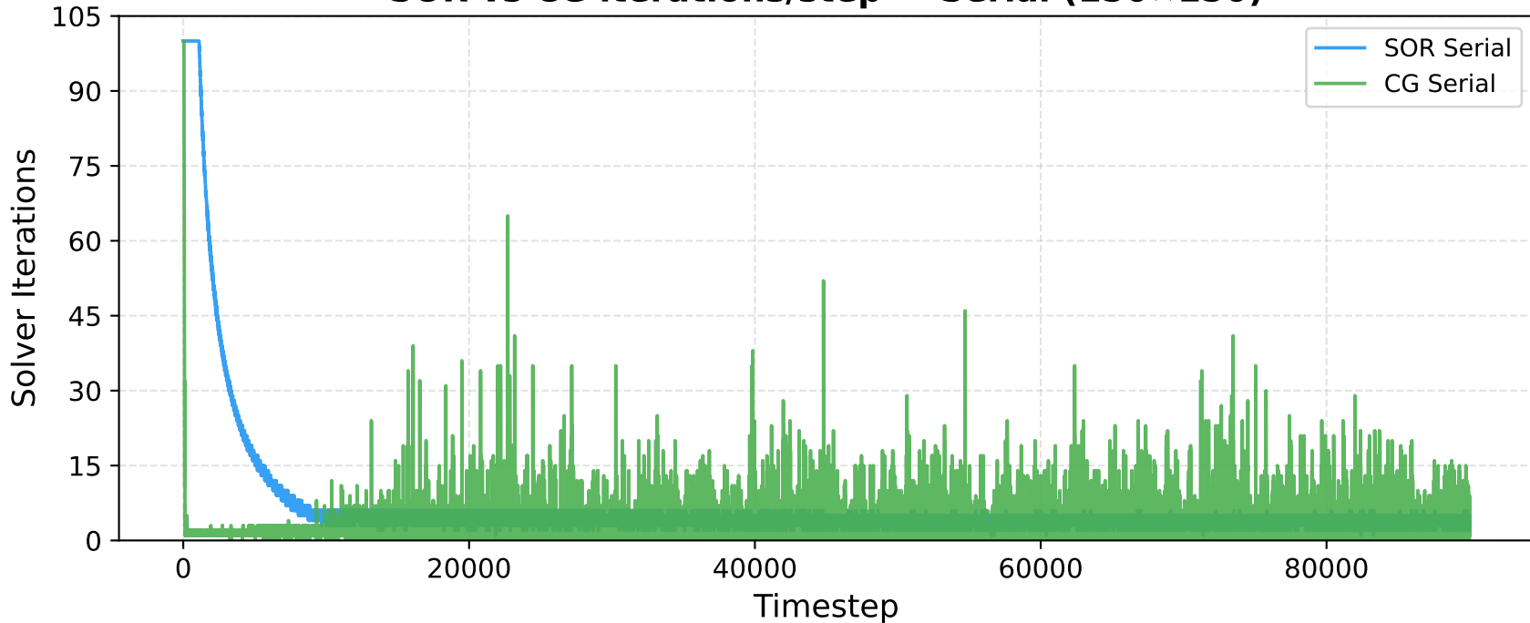
SOR vs CG iterations/step — Serial (150×150)
