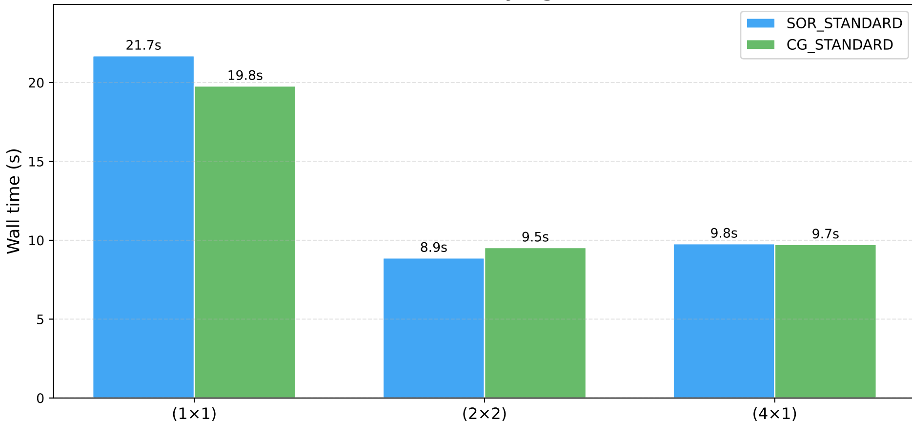
Wall time: SOR vs CG — Rayleigh-Bénard (40×18)
