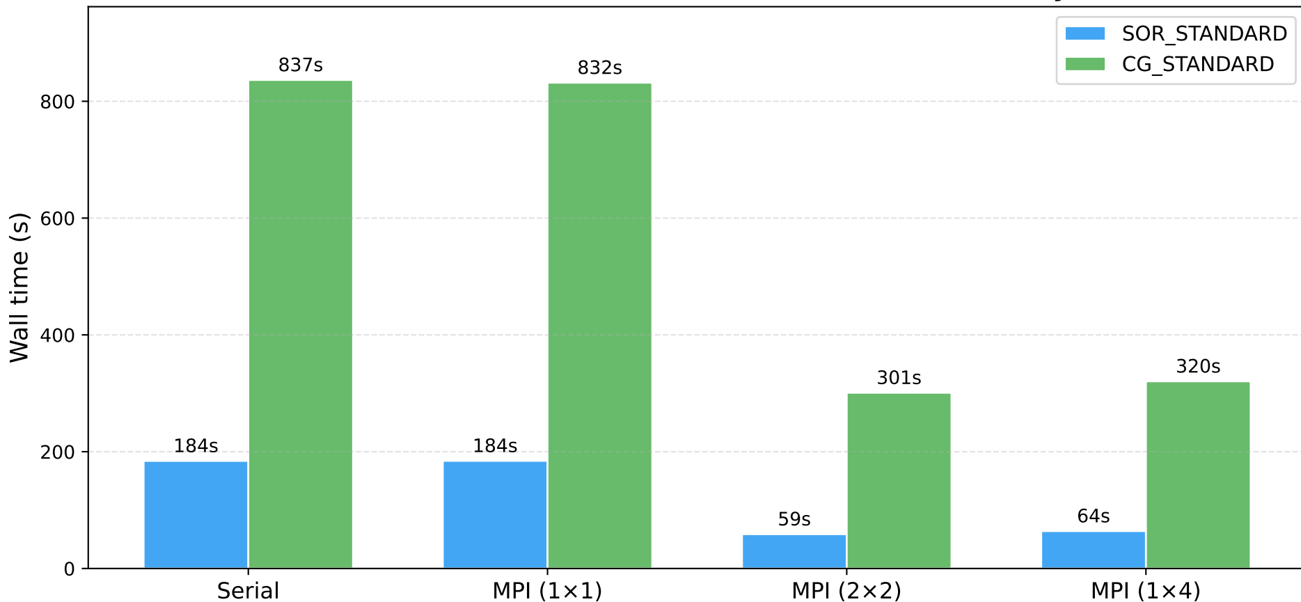
Wall time: SOR vs CG — 150×150 Lid-Driven Cavity
