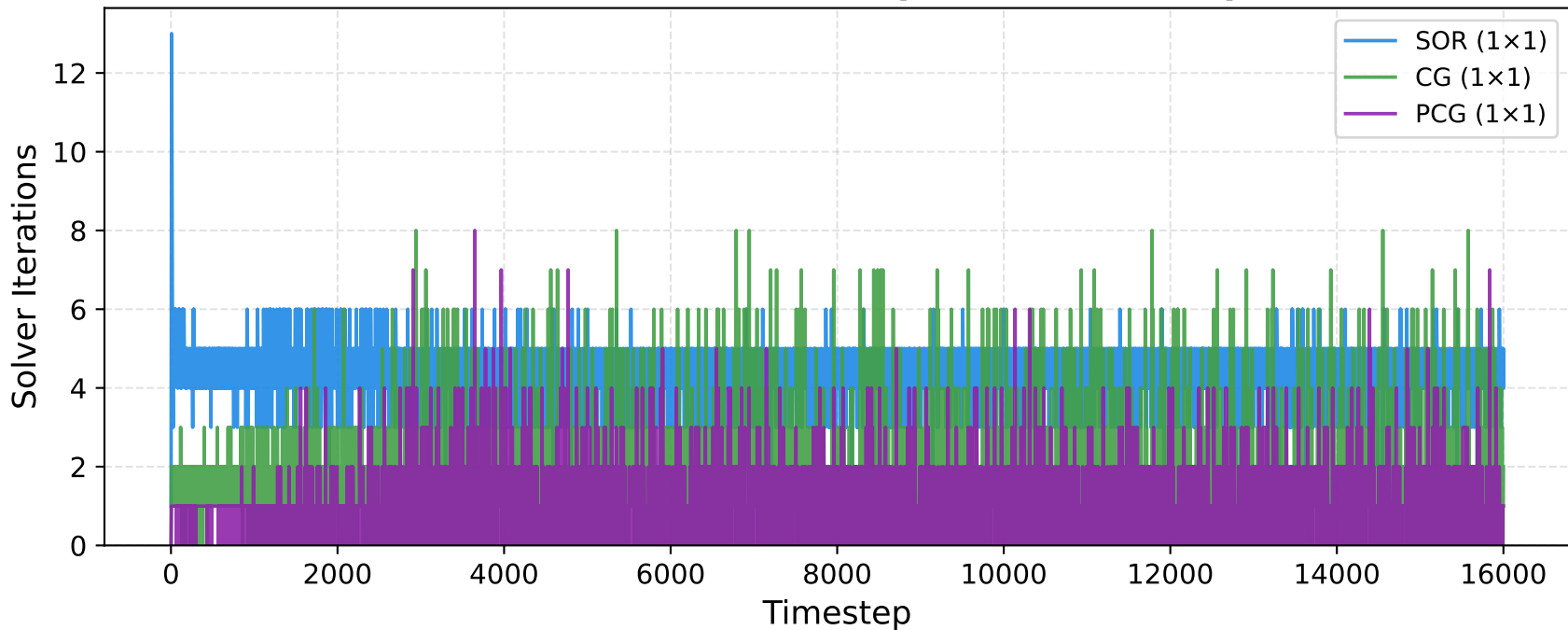
SOR vs CG vs PCG — iterations/step (1×1, Fluid Trap 200×100)
