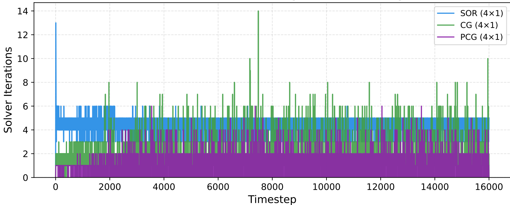
SOR vs CG vs PCG — iterations/step (4×1, Fluid Trap 200×100)
