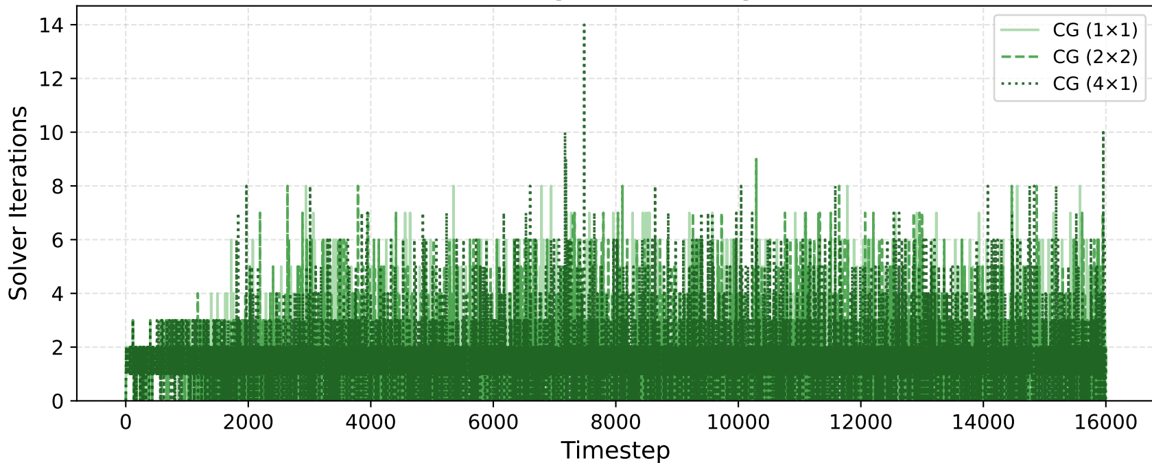
CG iterations/step — Fluid Trap (200×100)
