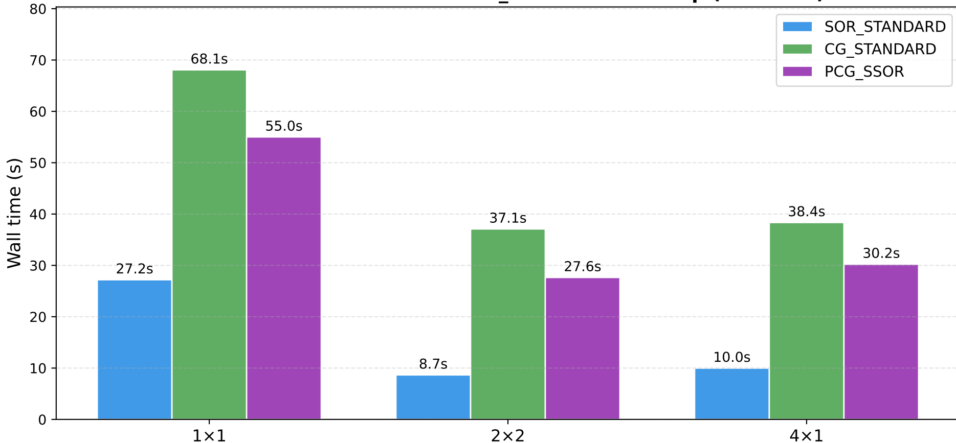
Wall time: SOR vs CG vs PCG_SSOR — Fluid Trap (200×100)
