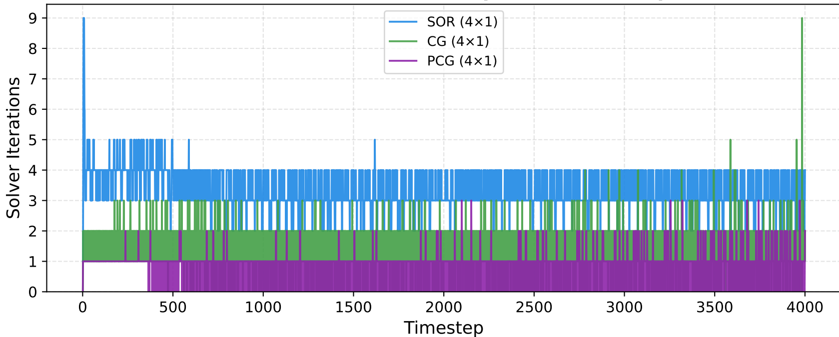
SOR vs CG vs PCG — iterations/step ( 4\times 1 , Fluid Trap 100\times 50 )
