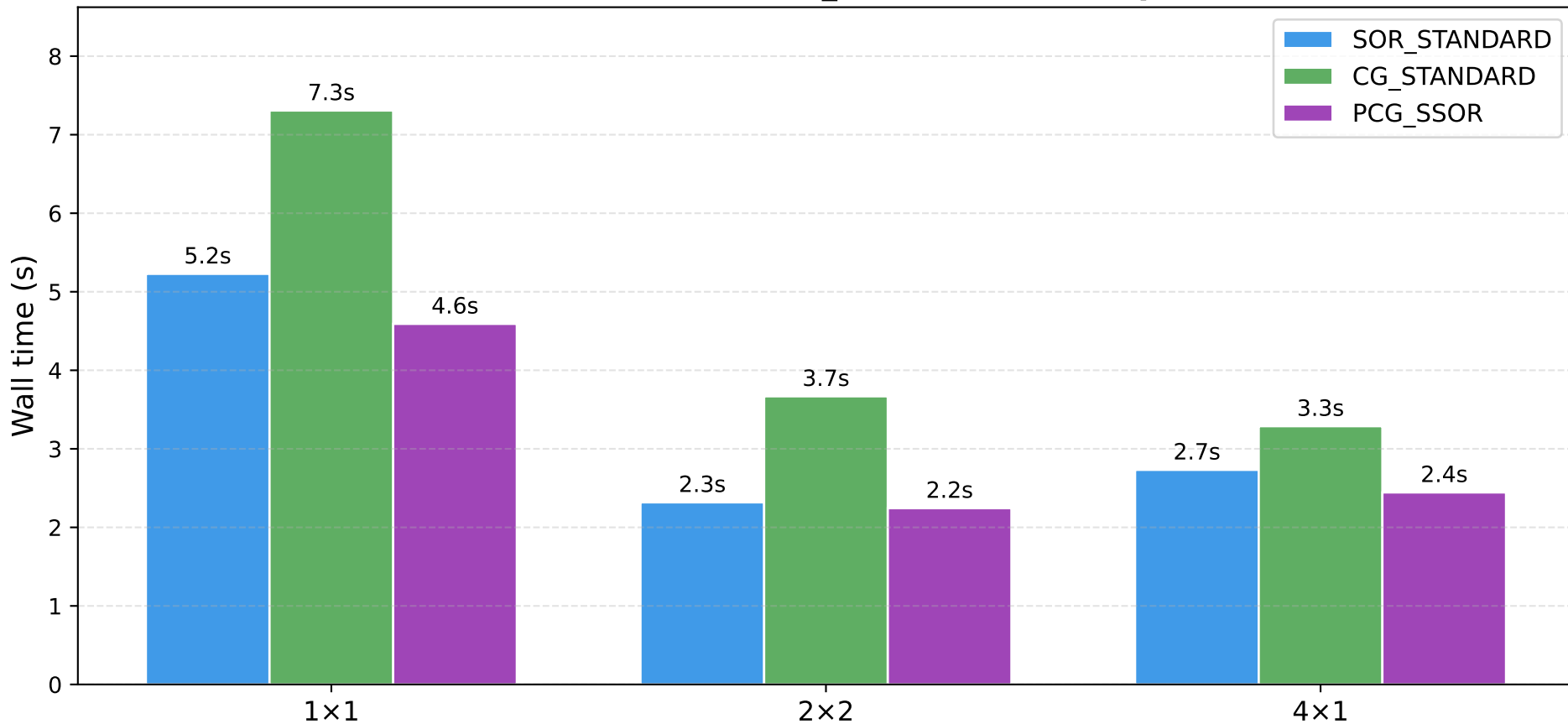
Wall time: SOR vs CG vs PCG_SSOR — Fluid Trap (100×50)
