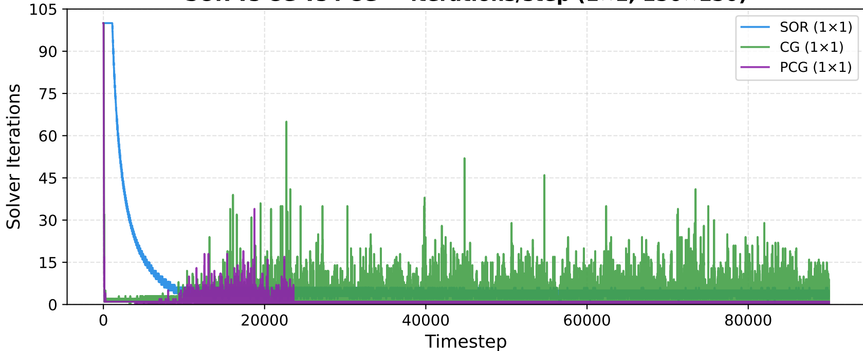
SOR vs CG vs PCG — iterations/step ( 1\times 1 , 150\times 150 )
