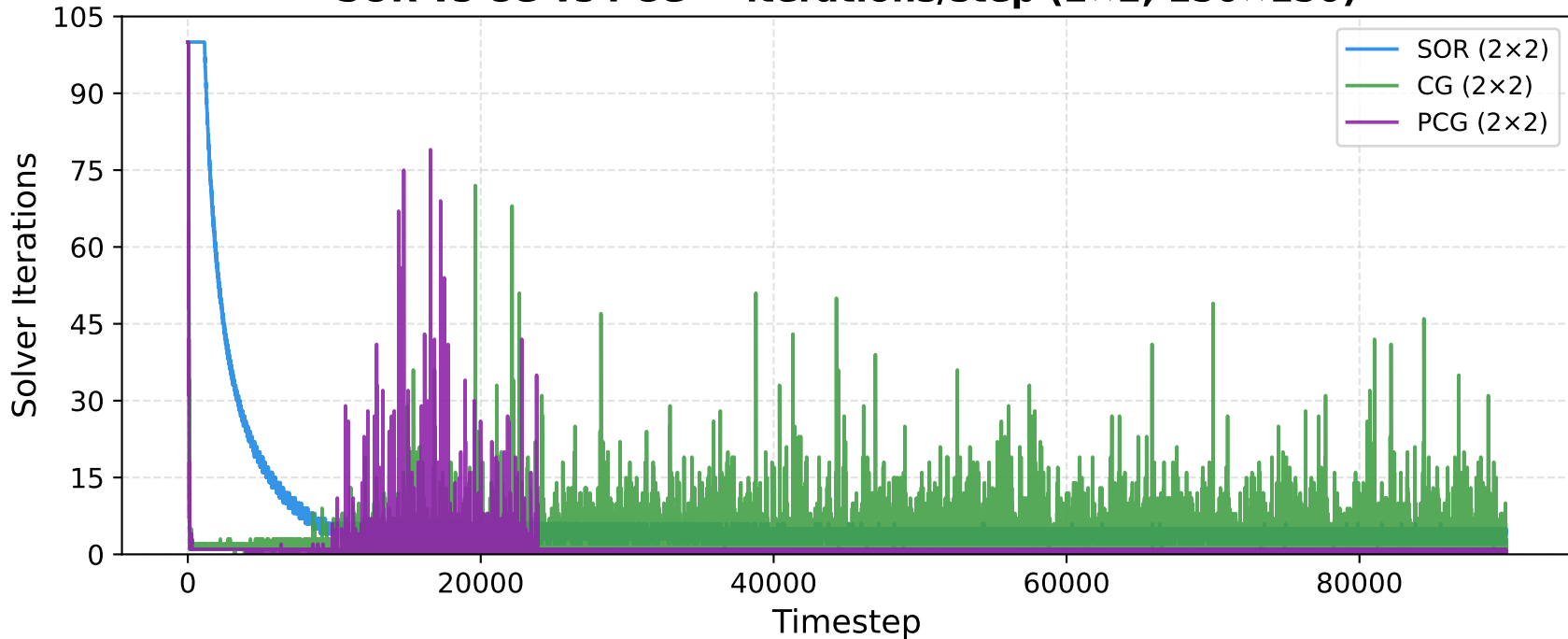
SOR vs CG vs PCG — iterations/step ( 2\times 2 , 150\times 150 )
