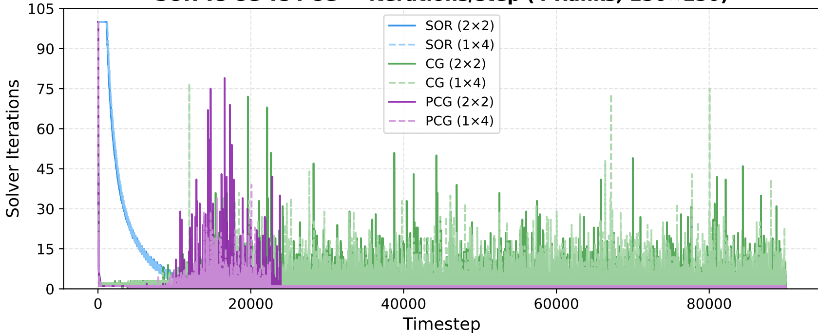
SOR vs CG vs PCG — iterations/step (4 Ranks, 150×150)
