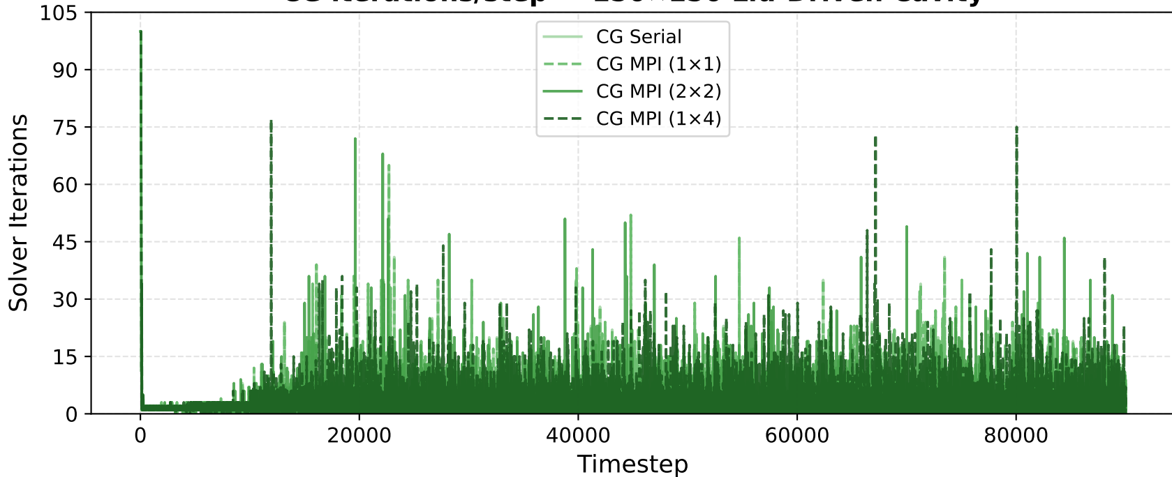
CG iterations/step — 150×150 Lid-Driven Cavity
