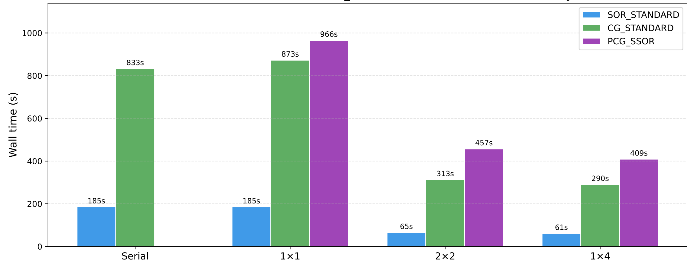
Wall time: SOR vs CG vs PCG_SSOR — 150×150 Lid-Driven Cavity
