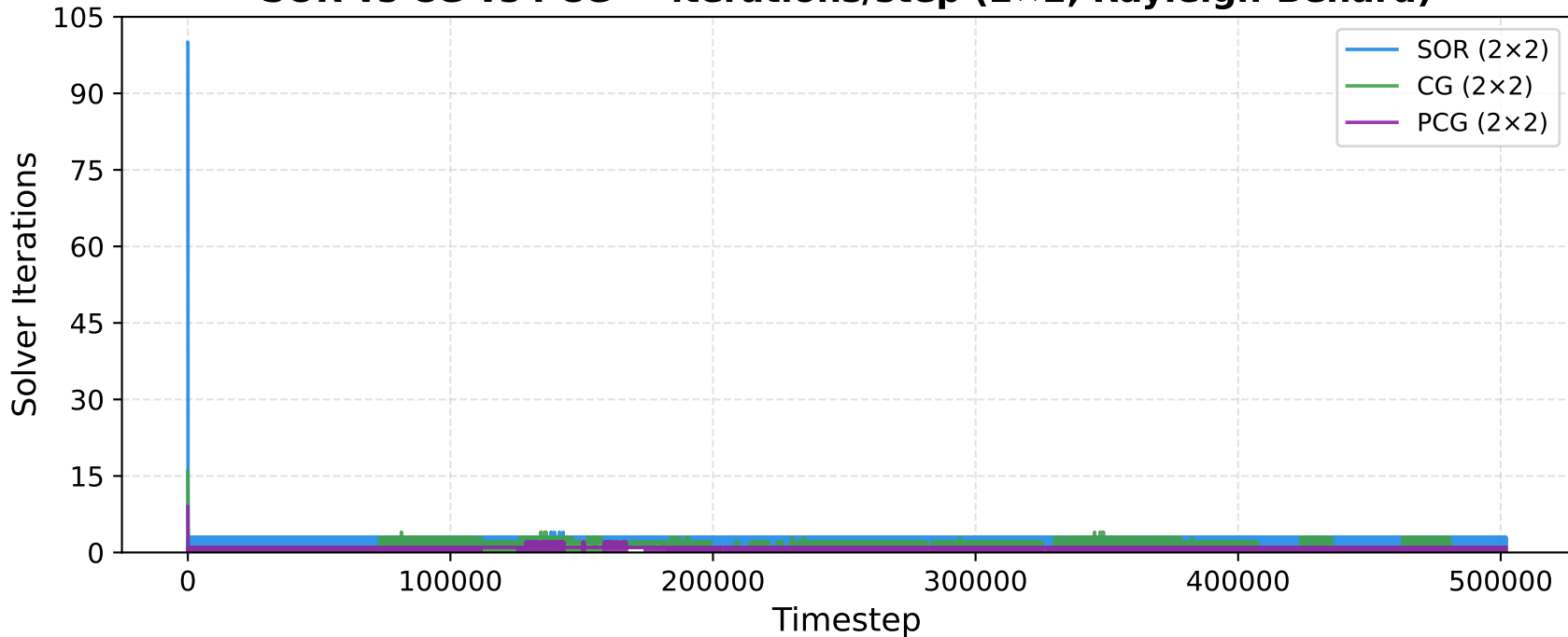
SOR vs CG vs PCG — iterations/step ( 2\times 2 , Rayleigh-Bénard)
