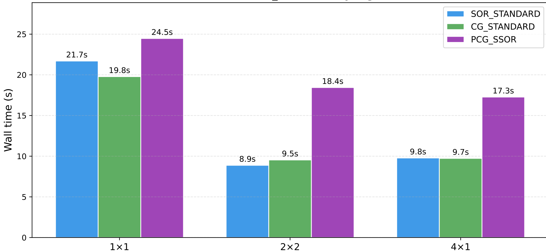
Wall time: SOR vs CG vs PCG_SSOR — Rayleigh-Bénard (40×18)
