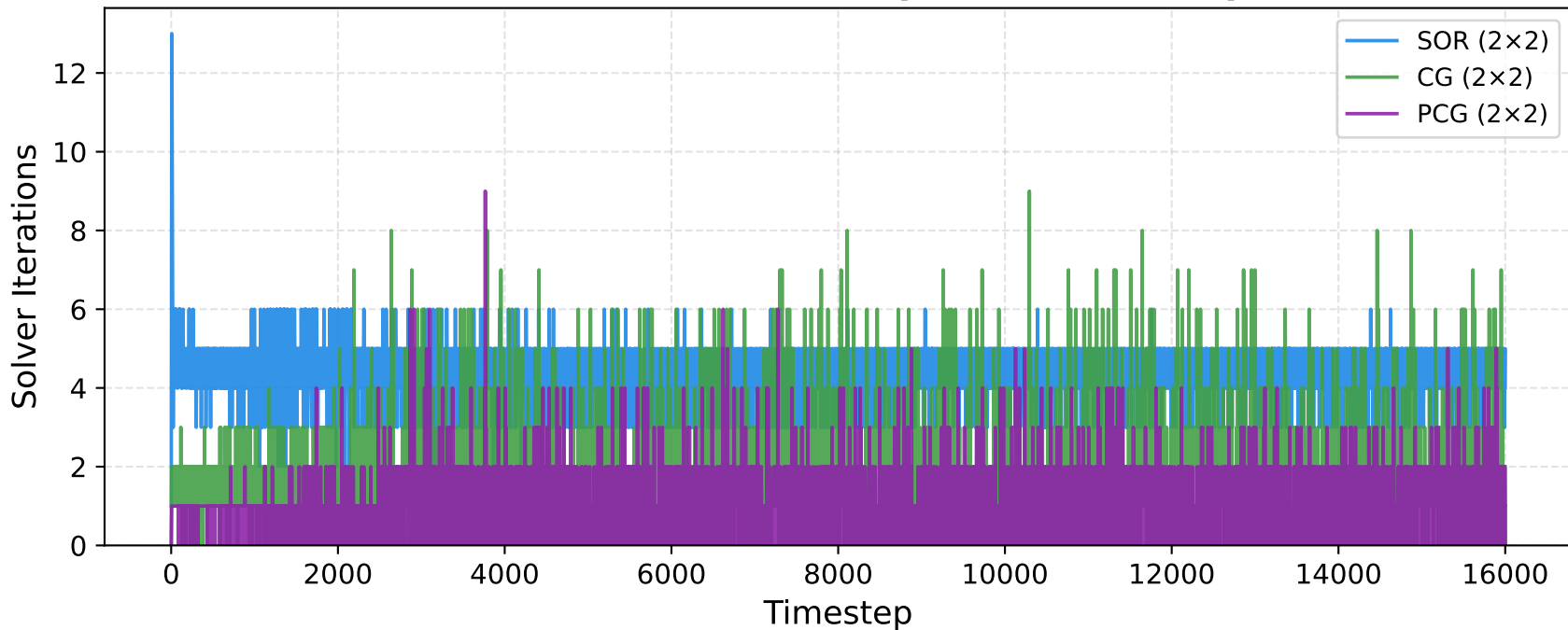
SOR vs CG vs PCG — iterations/step (2×2, Fluid Trap 200×100)
