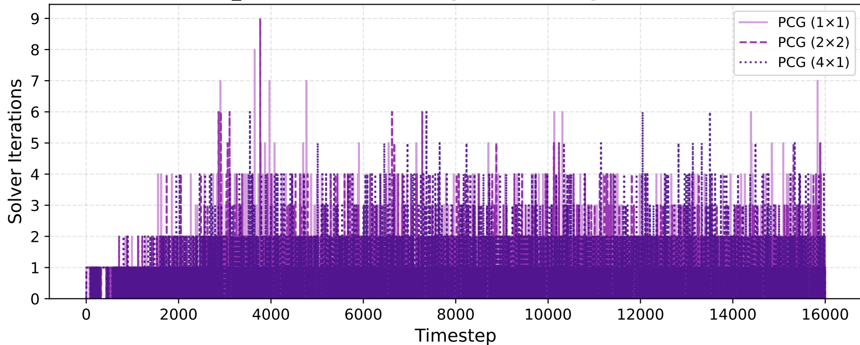
PCG_SSOR iterations/step — Fluid Trap (200×100)
