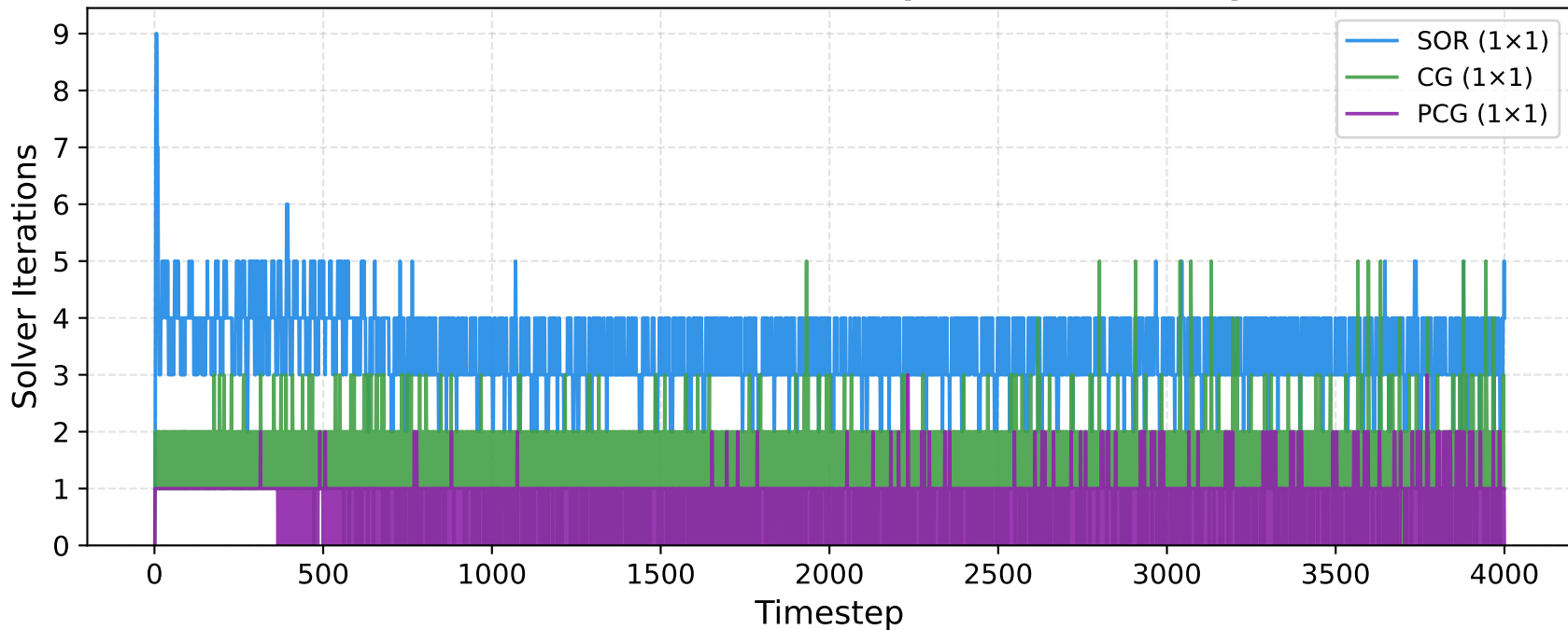
SOR vs CG vs PCG — iterations/step ( 1\times 1 , Fluid Trap 100\times 50 )
