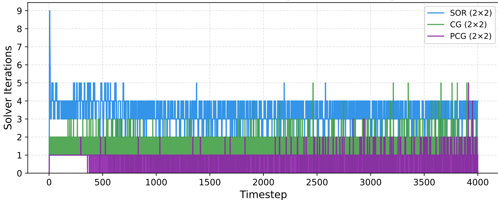
SOR vs CG vs PCG — iterations/step ( 2\times 2 , Fluid Trap 100\times 50 )
