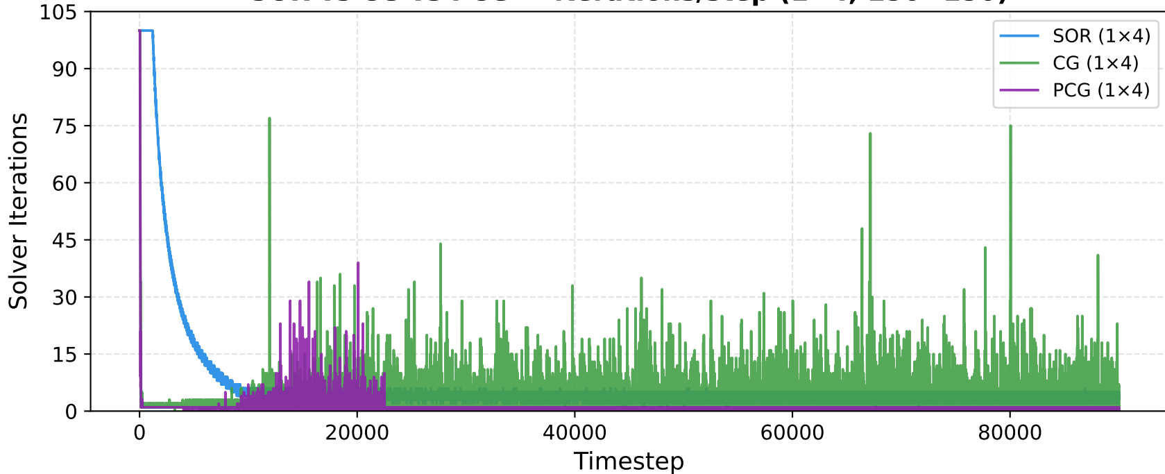
SOR vs CG vs PCG — iterations/step ( 1\times 4 , 150\times 150 )
