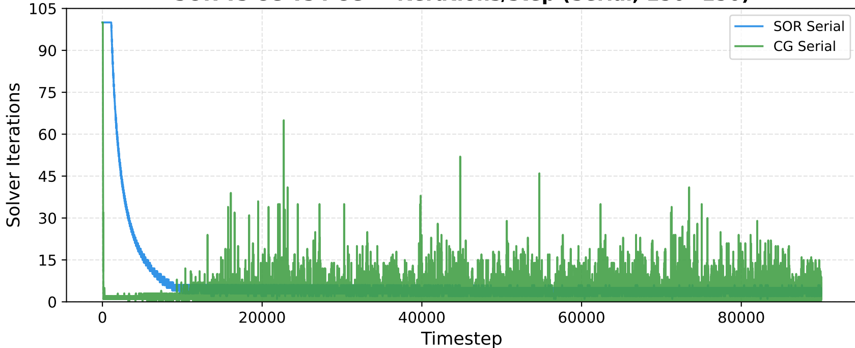
SOR vs CG vs PCG — iterations/step (Serial, 150×150)
