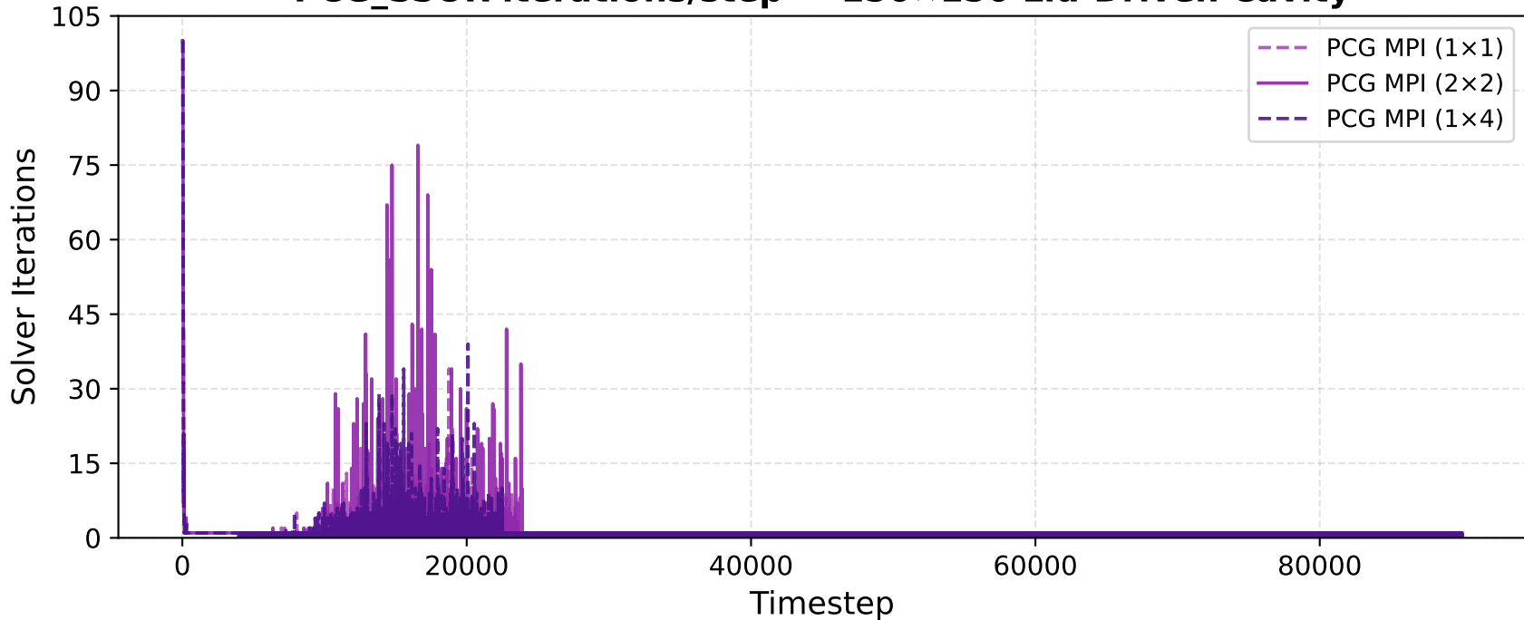
PCG_SSOR iterations/step — 150×150 Lid-Driven Cavity
