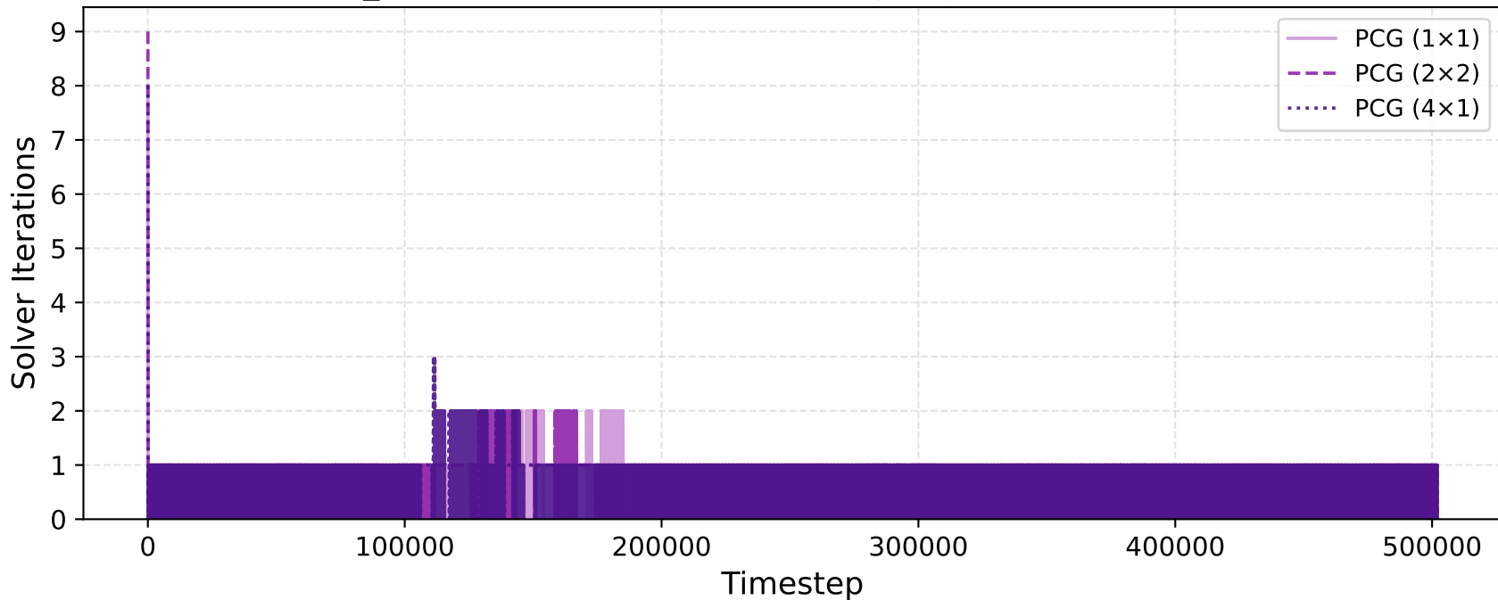
PCG_SSOR iterations/step — Rayleigh-Bénard (40×18)
