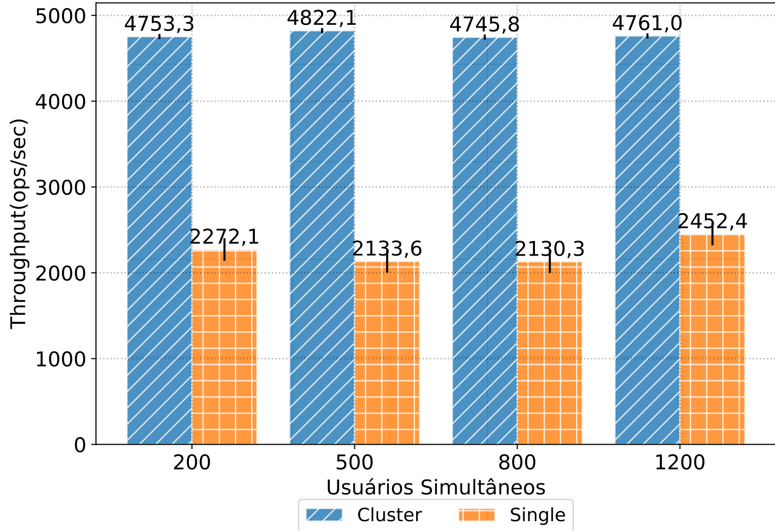
Performance ArangoDB Single x Cluster
