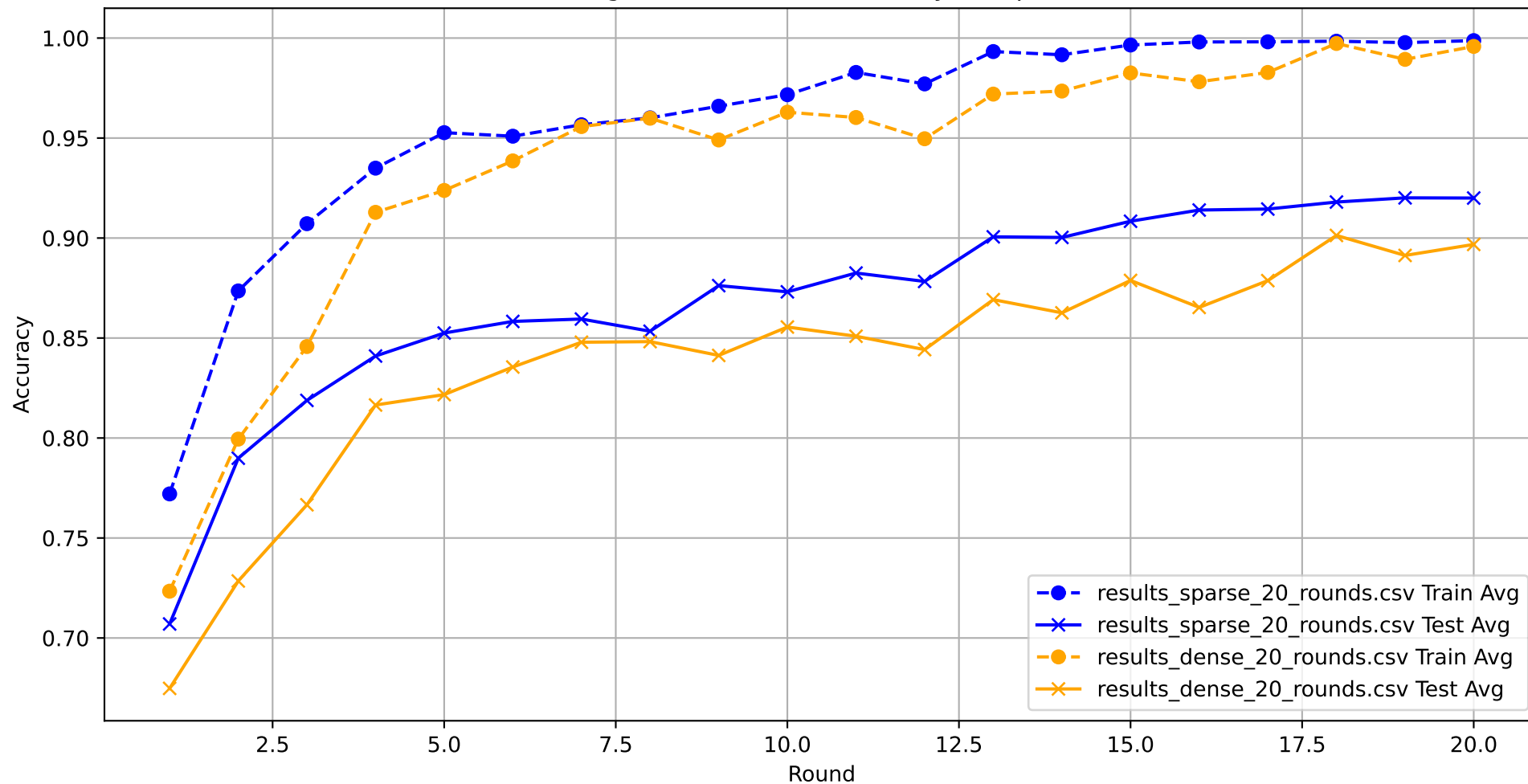
Average Train and Test Accuracy Comparison
