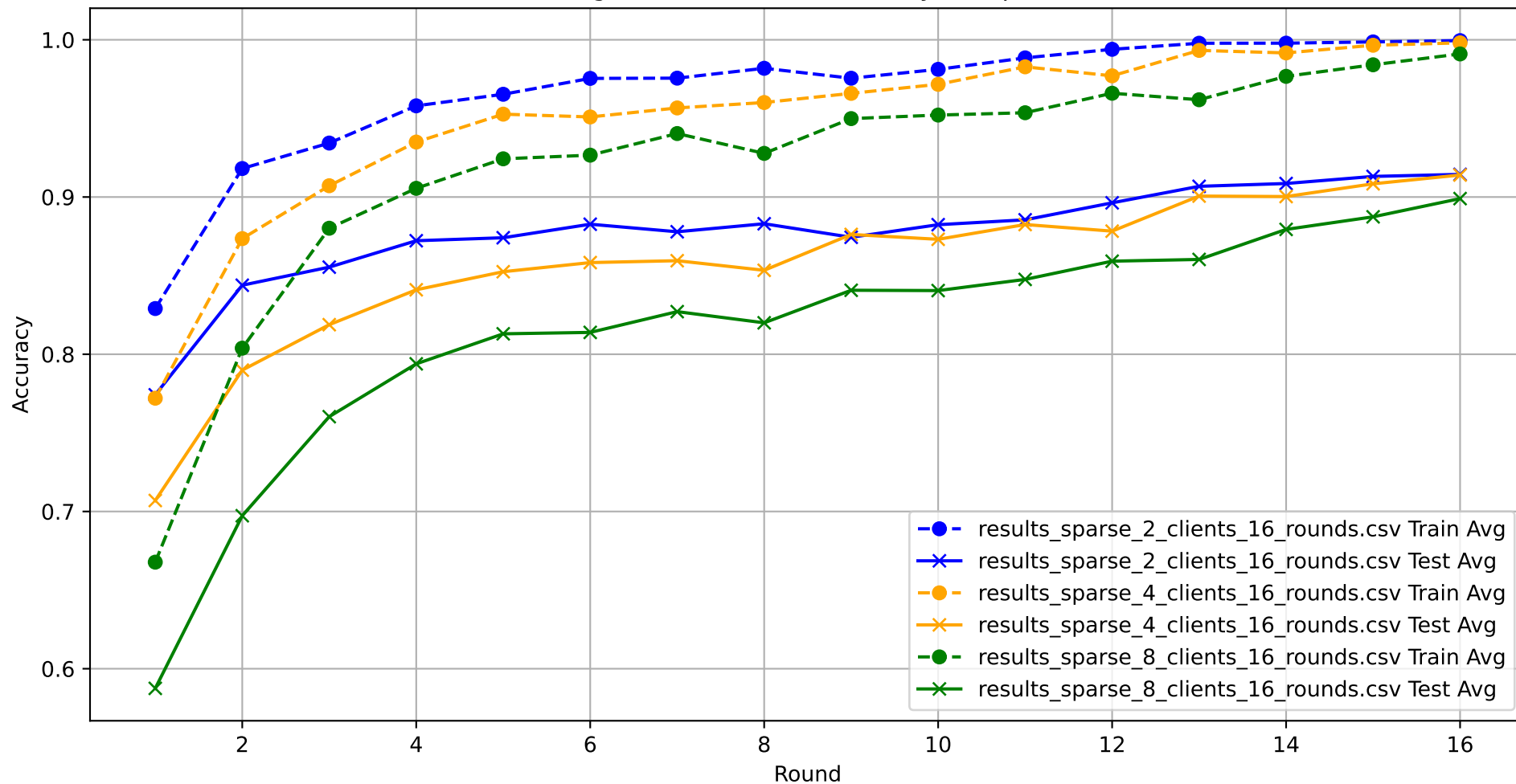
Average Train and Test Accuracy Comparison
