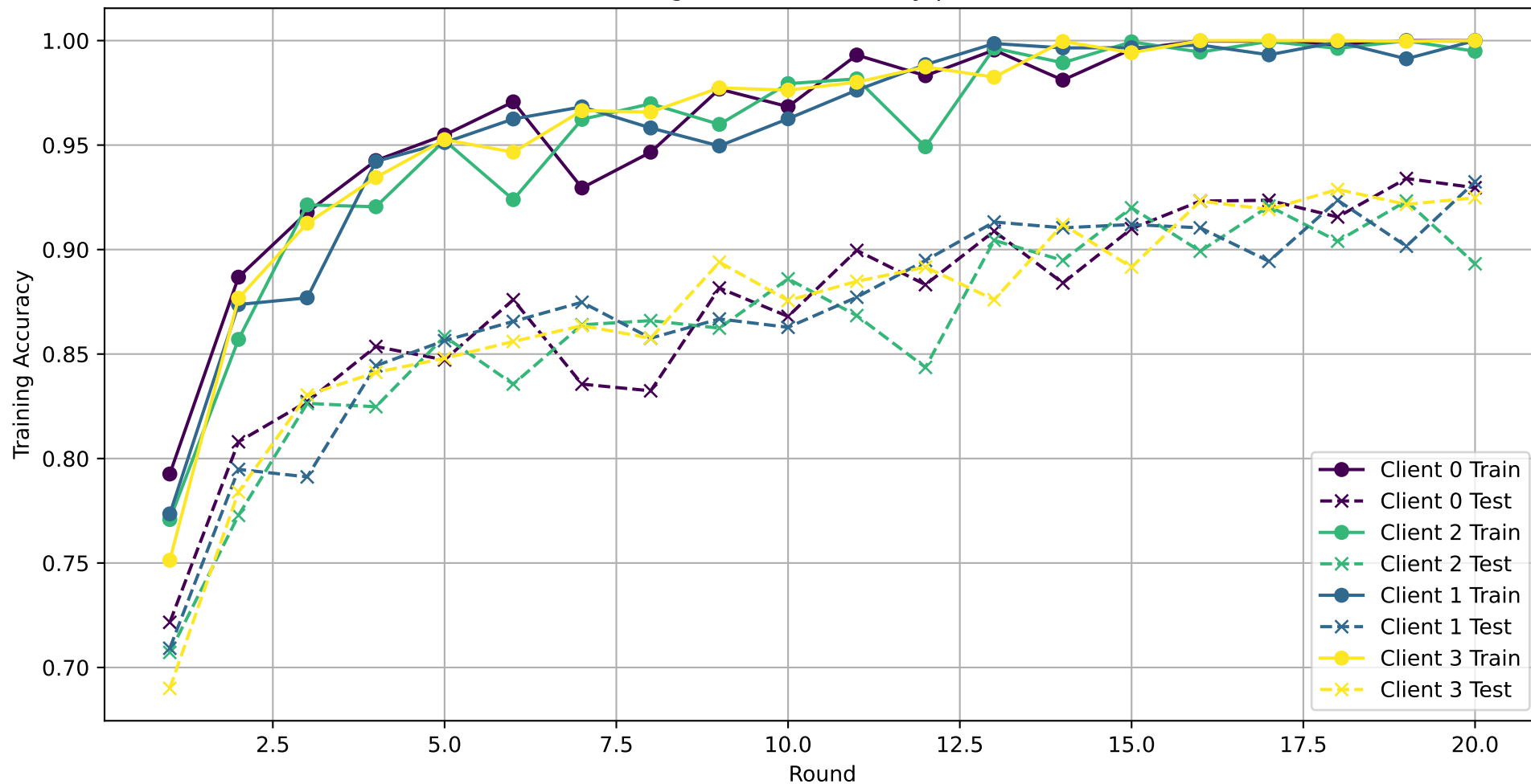
Training and Test Accuracy per Client
