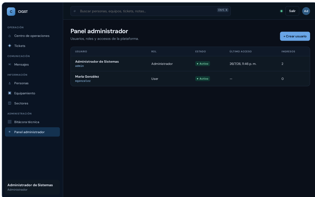
Panel administrador
