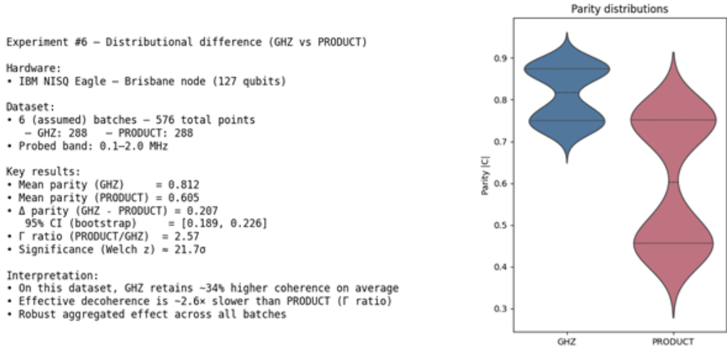
Figure 3.8: Distributional separation. Violin plots of parity outcomes ( n_{\text{obs}} = 576 ) show a statistically significant gap ( 21\sigma ) between GHZ (blue, protected) and product states (red, decaying).
