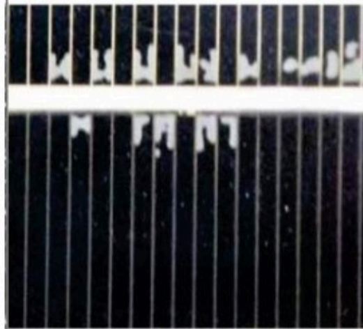
Encapsulant delamination from cell along grid fingers and bus bar [Packard12].
