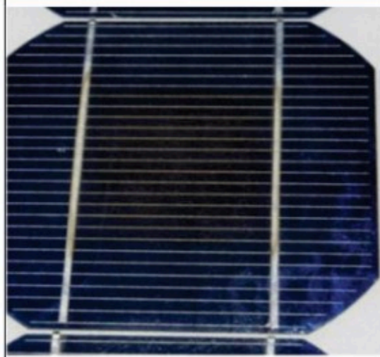
Slightly browned EVA in the centre of the cell with photobleaching at the edges [Köntges14].
