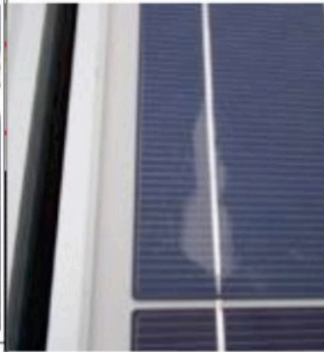
Encapsulant delamination along a bus-bar in a cell close to the module edge [Moser17].
